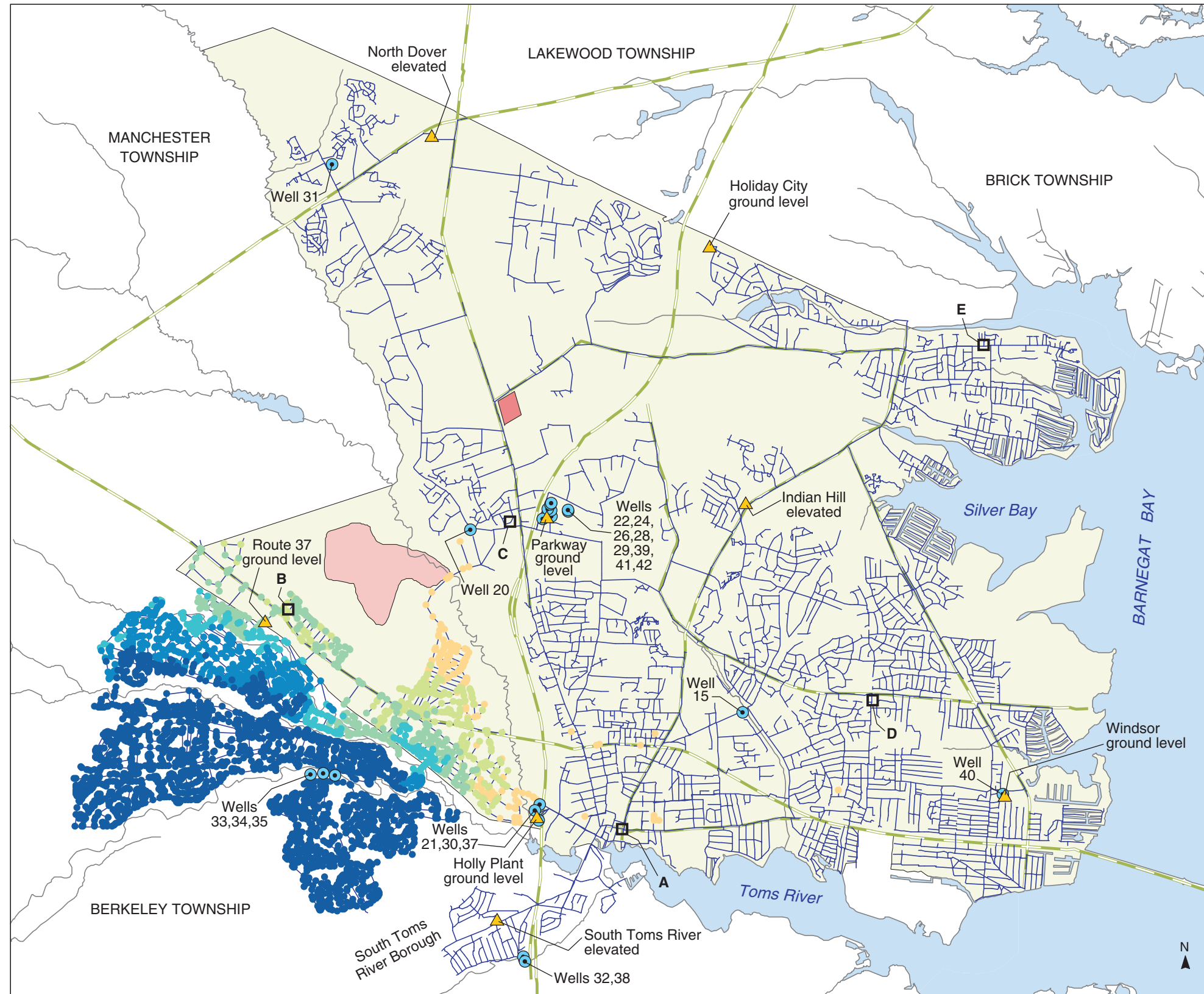
PLATE 129. AREAL DISTRIBUTION OF SIMULATED PROPORTIONATE CONTRIBUTION OF WATER FROM THE BERKELEY WELLS (33, 34, 35) TO LOCATIONS IN THE DOVER TOWNSHIP AREA, NEW JERSEY, AUGUST 1995 CONDITIONS By Morris L. Maslia, Jason B. Sautner, Mustafa M. Aral, Richard E. Gillig, Juan J. Reyes, and Robert C. Williams
