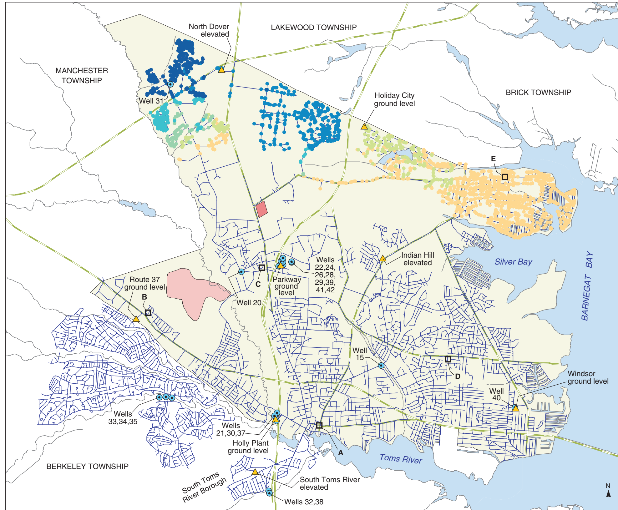
PLATE 128. AREAL DISTRIBUTION OF SIMULATED PROPORTIONATE CONTRIBUTION OF WATER FROM THE ROUTE 70 WELL (31) TO LOCATIONS IN THE DOVER TOWNSHIP AREA, NEW JERSEY, AUGUST 1995 CONDITIONS By Morris L. Maslia, Jason B. Sautner, Mustafa M. Aral, Richard E. Gillig, Juan J. Reyes, and Robert C. Williams
