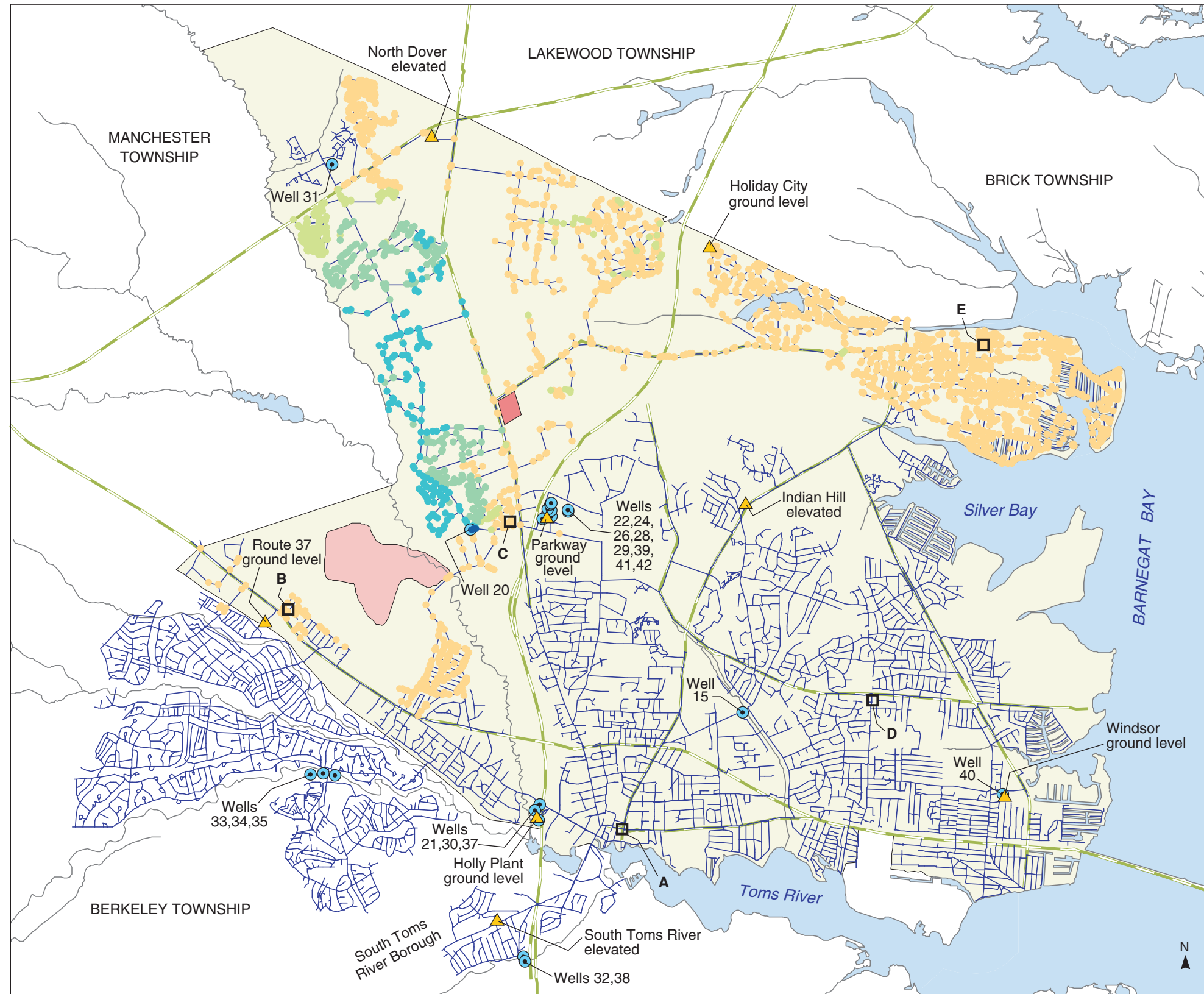
PLATE 126. AREAL DISTRIBUTION OF SIMULATED PROPORTIONATE CONTRIBUTION OF WATER FROM THE INDIAN HEAD WELL (20) TO LOCATIONS IN THE DOVER TOWNSHIP AREA, NEW JERSEY, AUGUST 1995 CONDITIONS By Morris L. Maslia, Jason B. Sautner, Mustafa M. Aral, Richard E. Gillig, Juan J. Reyes, and Robert C. Williams
