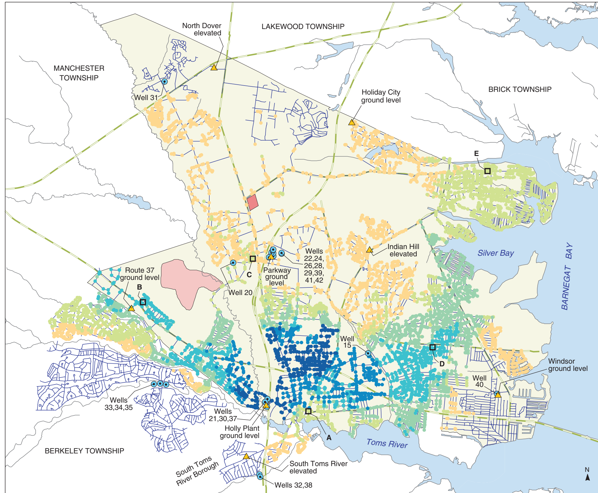
PLATE 123. AREAL DISTRIBUTION OF SIMULATED PROPORTIONATE CONTRIBUTION OF WATER FROM THE HOLLY WELLS (21, 30, 37) TO LOCATIONS IN THE DOVER TOWNSHIP AREA, NEW JERSEY, AUGUST 1995 CONDITIONS By Morris L. Maslia, Jason B. Sautner, Mustafa M. Aral, Richard E. Gillig, Juan J. Reyes, and Robert C. Williams
