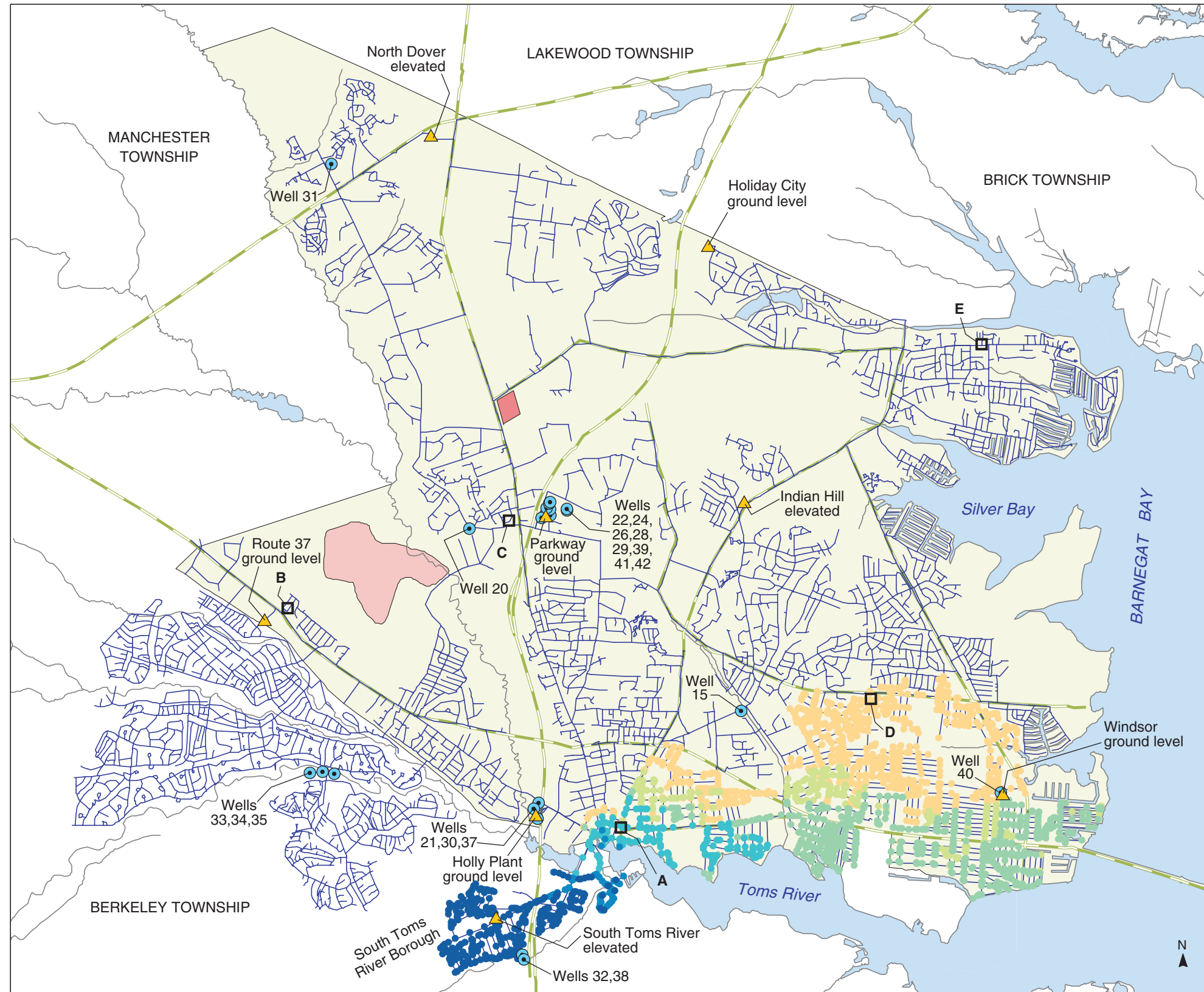
PLATE 118. AREAL DISTRIBUTION OF SIMULATED PROPORTIONATE CONTRIBUTION OF WATER FROM THE SOUTH TOMS RIVER WELL (32) TO LOCATIONS IN THE DOVER TOWNSHIP AREA, NEW JERSEY, FEBRUARY 1995 CONDITIONS
