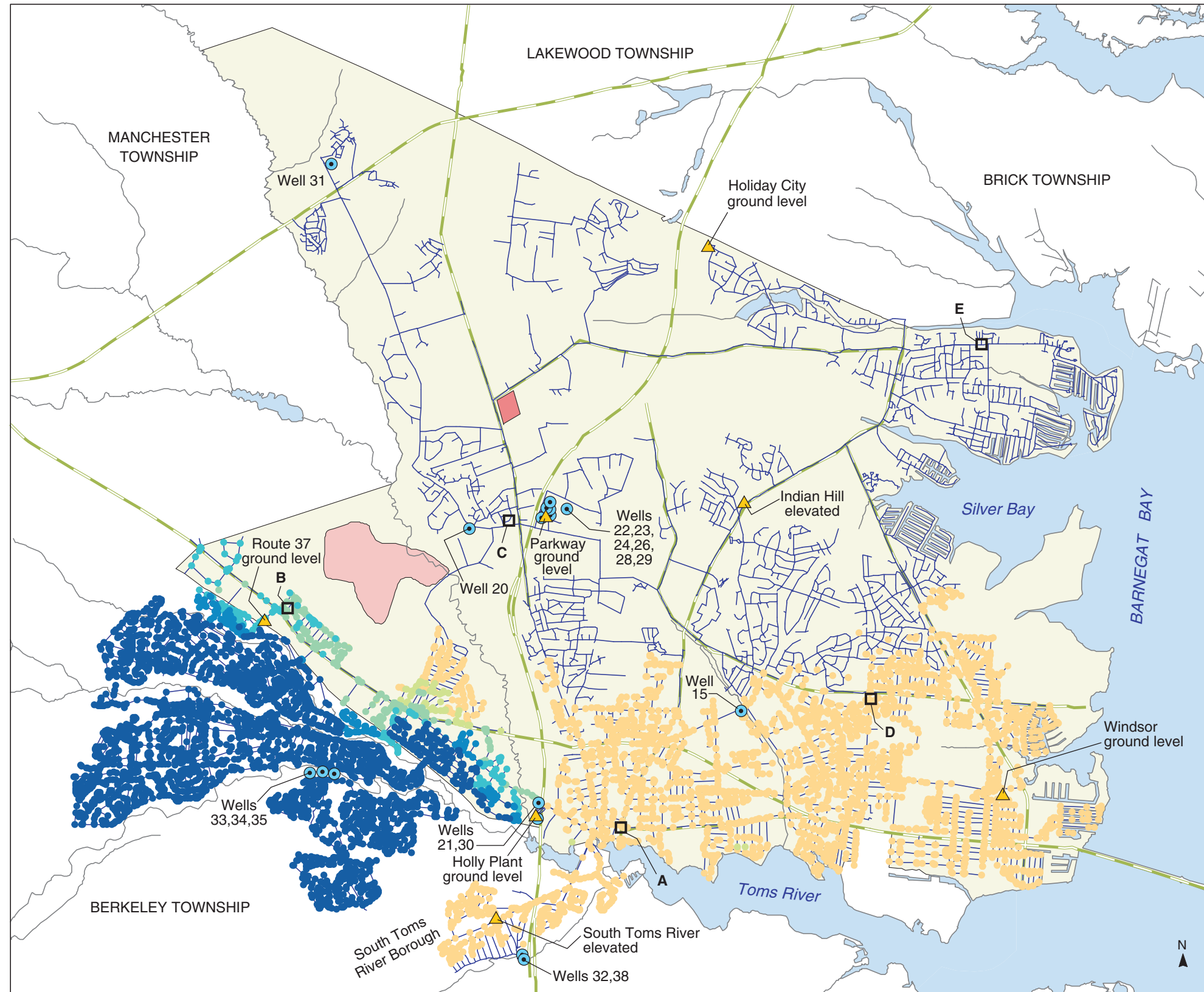
PLATE 117. AREAL DISTRIBUTION OF SIMULATED PROPORTIONATE CONTRIBUTION OF WATER FROM THE BERKELEY WELLS (33, 34, 35) TO LOCATIONS IN THE DOVER TOWNSHIP AREA, NEW JERSEY, OCTOBER 1988 CONDITIONS By Morris L. Maslia, Jason B. Sautner, Mustafa M. Aral, Richard E. Gillig, Juan J. Reyes, and Robert C. Williams
