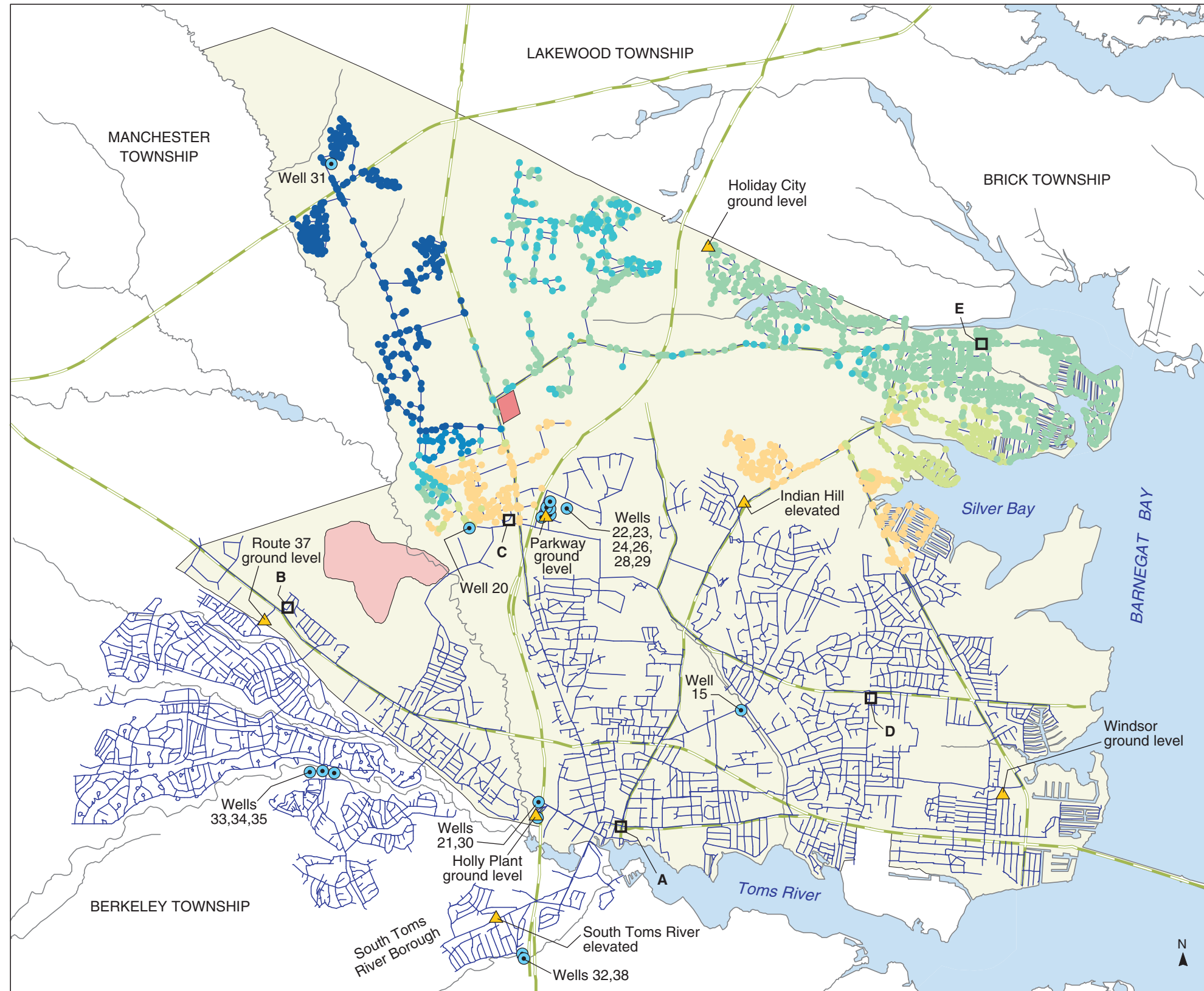
PLATE 116. AREAL DISTRIBUTION OF SIMULATED PROPORTIONATE CONTRIBUTION OF WATER FROM THE ROUTE 70 WELL (31) TO LOCATIONS IN THE DOVER TOWNSHIP AREA, NEW JERSEY, OCTOBER 1988 CONDITIONS By Morris L. Maslia, Jason B. Sautner, Mustafa M. Aral, Richard E. Gillig, Juan J. Reyes, and Robert C. Williams
