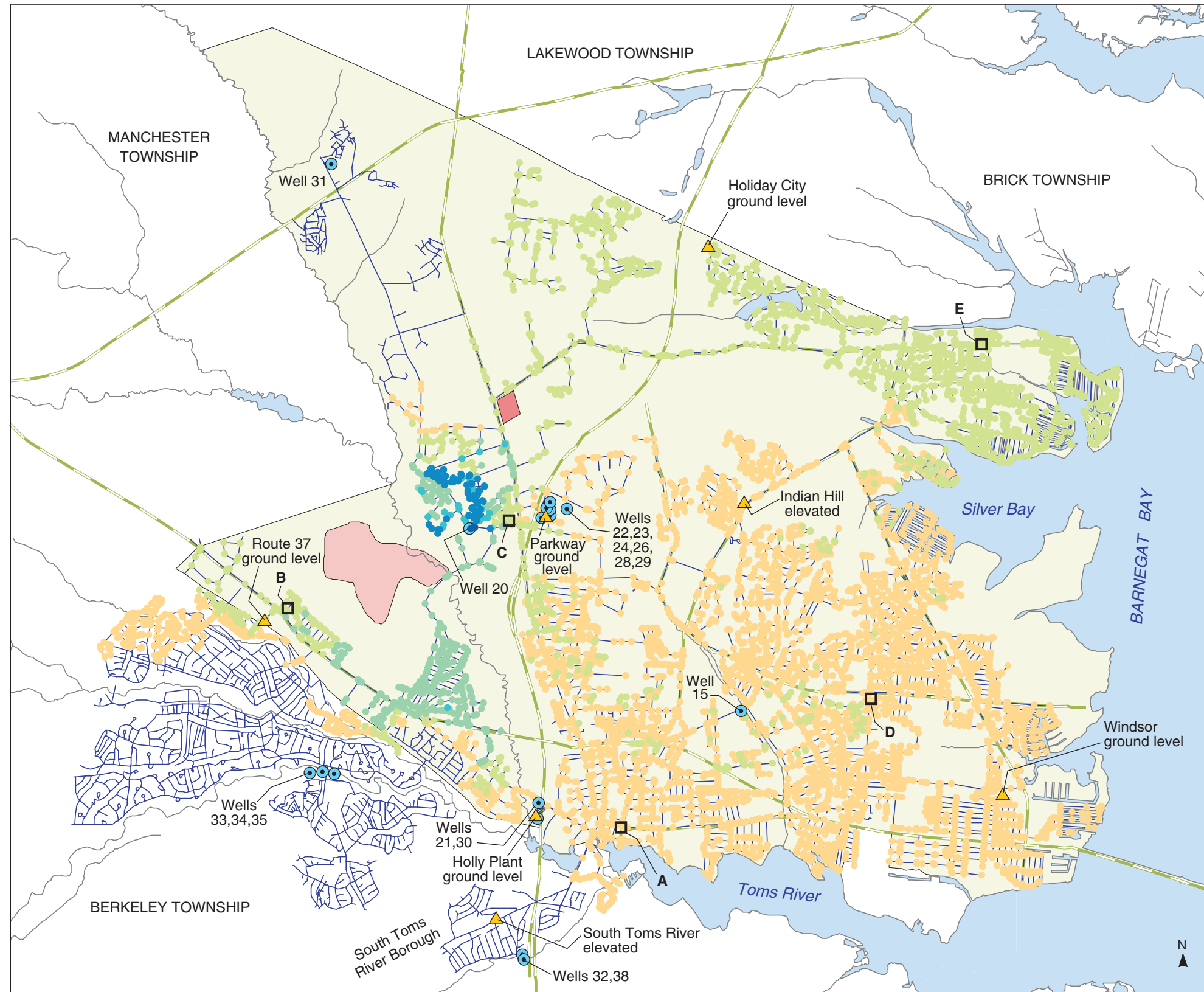
PLATE 114. AREAL DISTRIBUTION OF SIMULATED PROPORTIONATE CONTRIBUTION OF WATER FROM THE INDIAN HEAD WELL (20) TO LOCATIONS IN THE DOVER TOWNSHIP AREA, NEW JERSEY, OCTOBER 1988 CONDITIONS By Morris L. Maslia, Jason B. Sautner, Mustafa M. Aral, Richard E. Gillig, Juan J. Reyes, and Robert C. Williams
