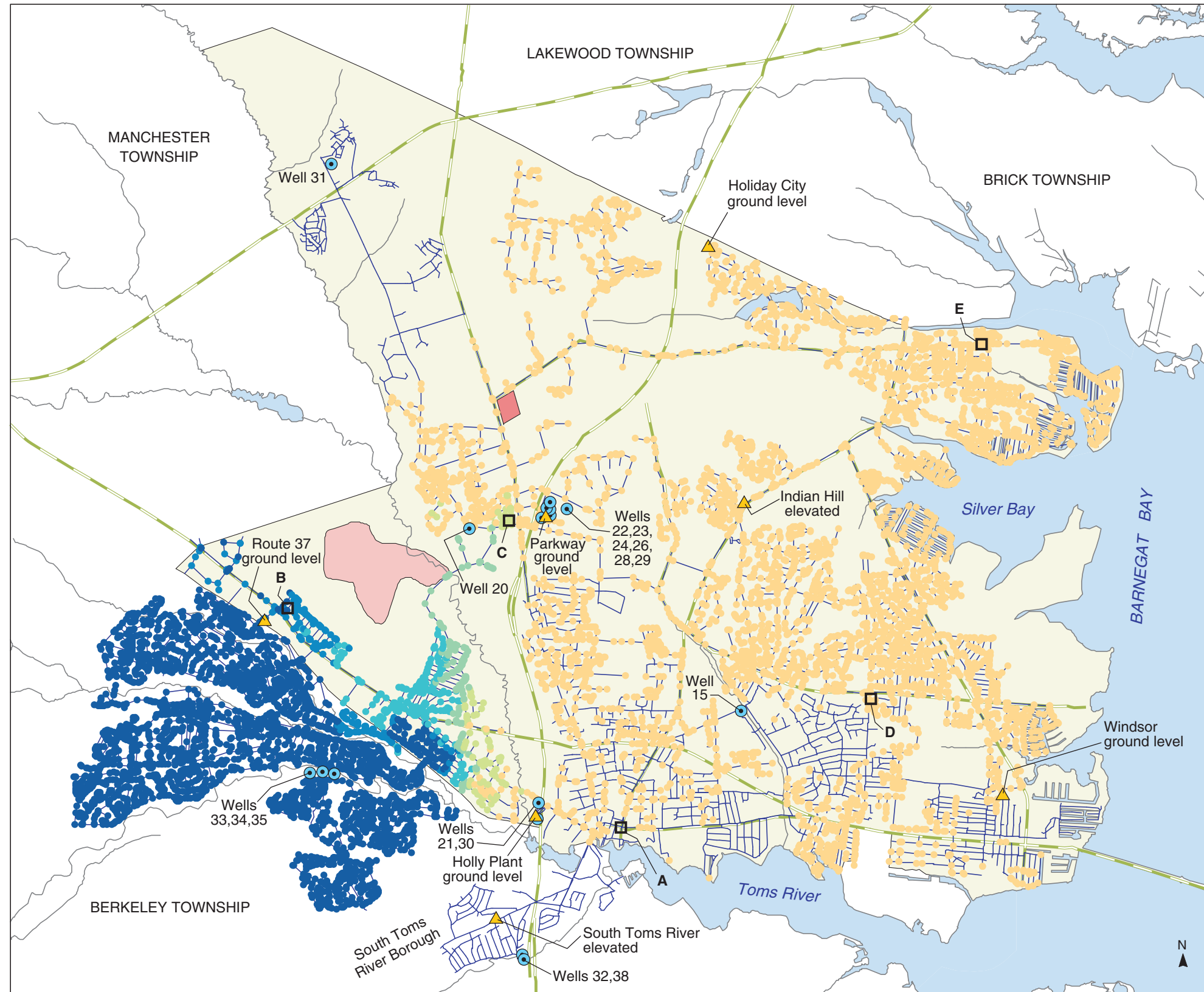
PLATE 111. AREAL DISTRIBUTION OF SIMULATED PROPORTIONATE CONTRIBUTION OF WATER FROM THE BERKELEY WELLS (33, 34, 35) TO LOCATIONS IN THE DOVER TOWNSHIP AREA, NEW JERSEY, JULY 1988 CONDITIONS By Morris L. Maslia, Jason B. Sautner, Mustafa M. Aral, Richard E. Gillig, Juan J. Reyes, and Robert C. Williams
