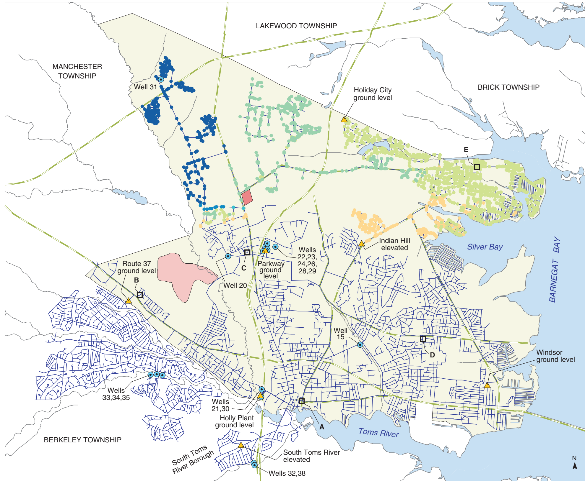
PLATE 110. AREAL DISTRIBUTION OF SIMULATED PROPORTIONATE CONTRIBUTION OF WATER FROM THE ROUTE 70 WELL (31) TO LOCATIONS IN THE DOVER TOWNSHIP AREA, NEW JERSEY, JULY 1988 CONDITIONS By Morris L. Maslia, Jason B. Sautner, Mustafa M. Aral, Richard E. Gillig, Juan J. Reyes, and Robert C. Williams
