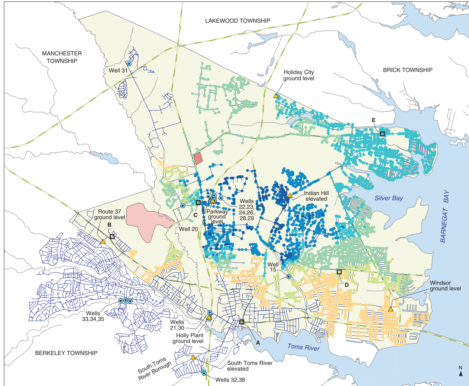
PLATE 109. AREAL DISTRIBUTION OF SIMULATED PROPORTIONATE CONTRIBUTION OF WATER FROM THE PARKWAY WELLS (22, 23, 24, 26, 28, 29) TO LOCATIONS IN THE DOVER TOWNSHIP AREA, NEW JERSEY, JULY 1988 CONDITIONS By Morris L. Maslia, Jason B. Sautner, Mustafa M. Aral, Richard E. Gillig, Juan J. Reyes, and Robert C. Williams
