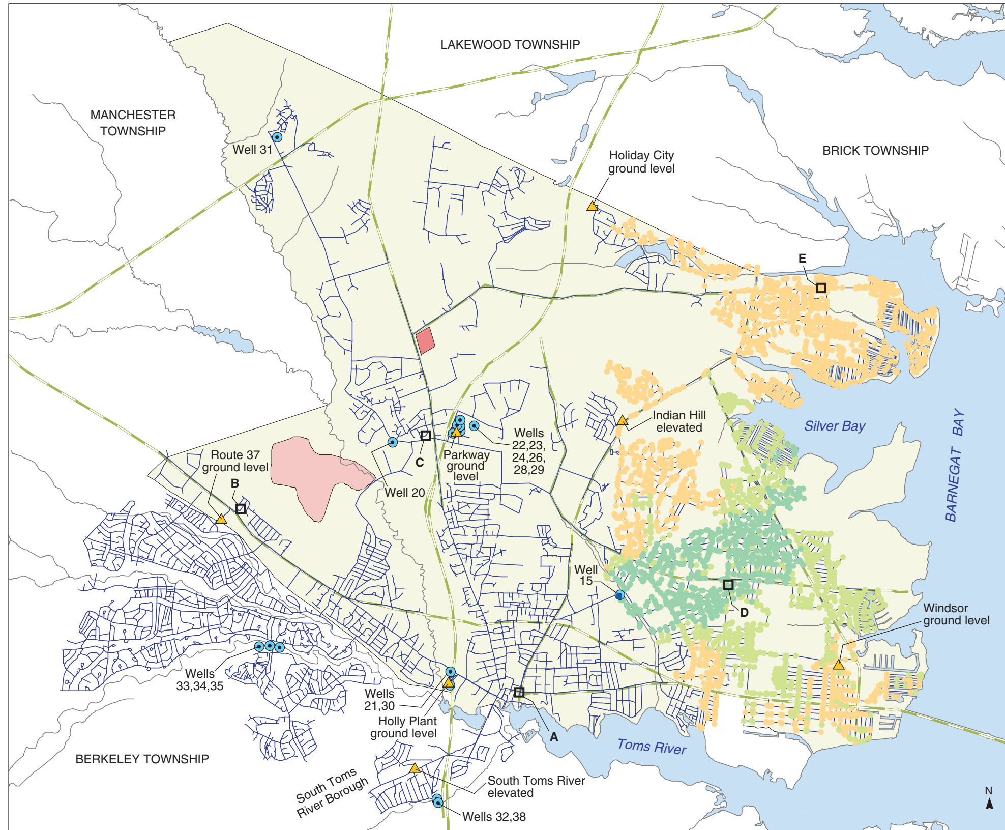
PLATE 106. AREAL DISTRIBUTION OF SIMULATED PROPORTIONATE CONTRIBUTION OF WATER FROM THE BROOKSIDE WELL (15) TO LOCATIONS IN THE DOVER TOWNSHIP AREA, NEW JERSEY, JULY 1988 CONDITIONS
