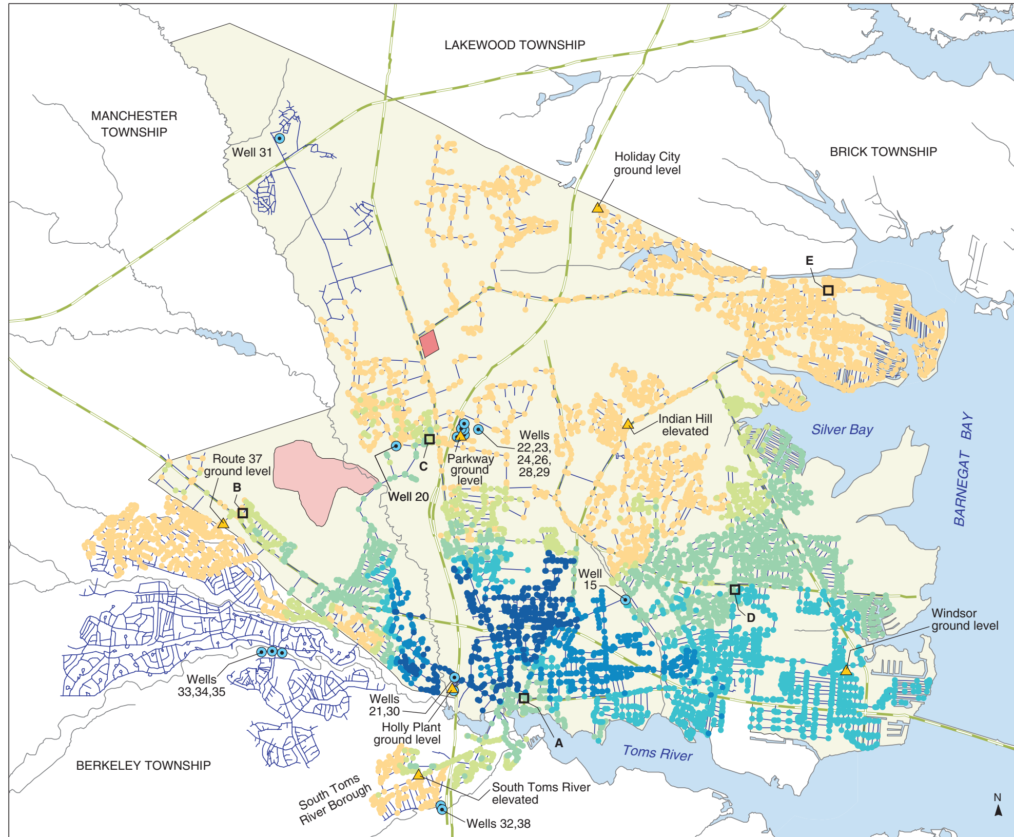
PLATE 105. AREAL DISTRIBUTION OF SIMULATED PROPORTIONATE CONTRIBUTION OF WATER FROM THE HOLLY WELLS (21, 30) TO LOCATIONS IN THE DOVER TOWNSHIP AREA, NEW JERSEY, JULY 1988 CONDITIONS By Morris L. Maslia, Jason B. Sautner, Mustafa M. Aral, Richard E. Gillig, Juan J. Reyes, and Robert C. Williams
