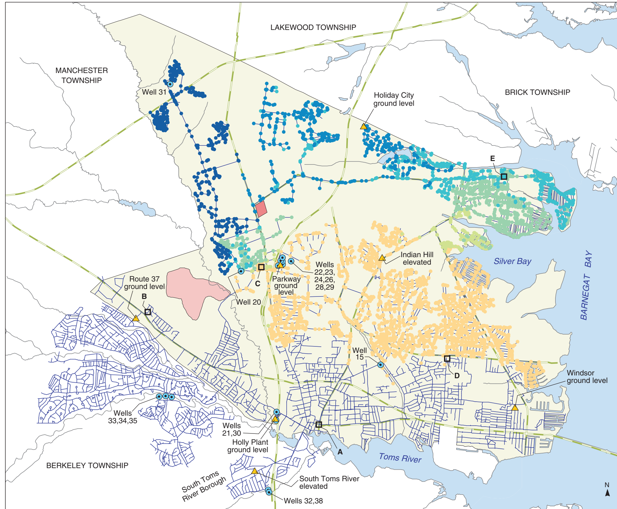
PLATE 103. AREAL DISTRIBUTION OF SIMULATED PROPORTIONATE CONTRIBUTION OF WATER FROM THE ROUTE 70 WELL (31) TO LOCATIONS IN THE DOVER TOWNSHIP AREA, NEW JERSEY, FEBRUARY 1988 CONDITIONS By Morris L. Maslia, Jason B. Sautner, Mustafa M. Aral, Richard E. Gillig, Juan J. Reyes, and Robert C. Williams
