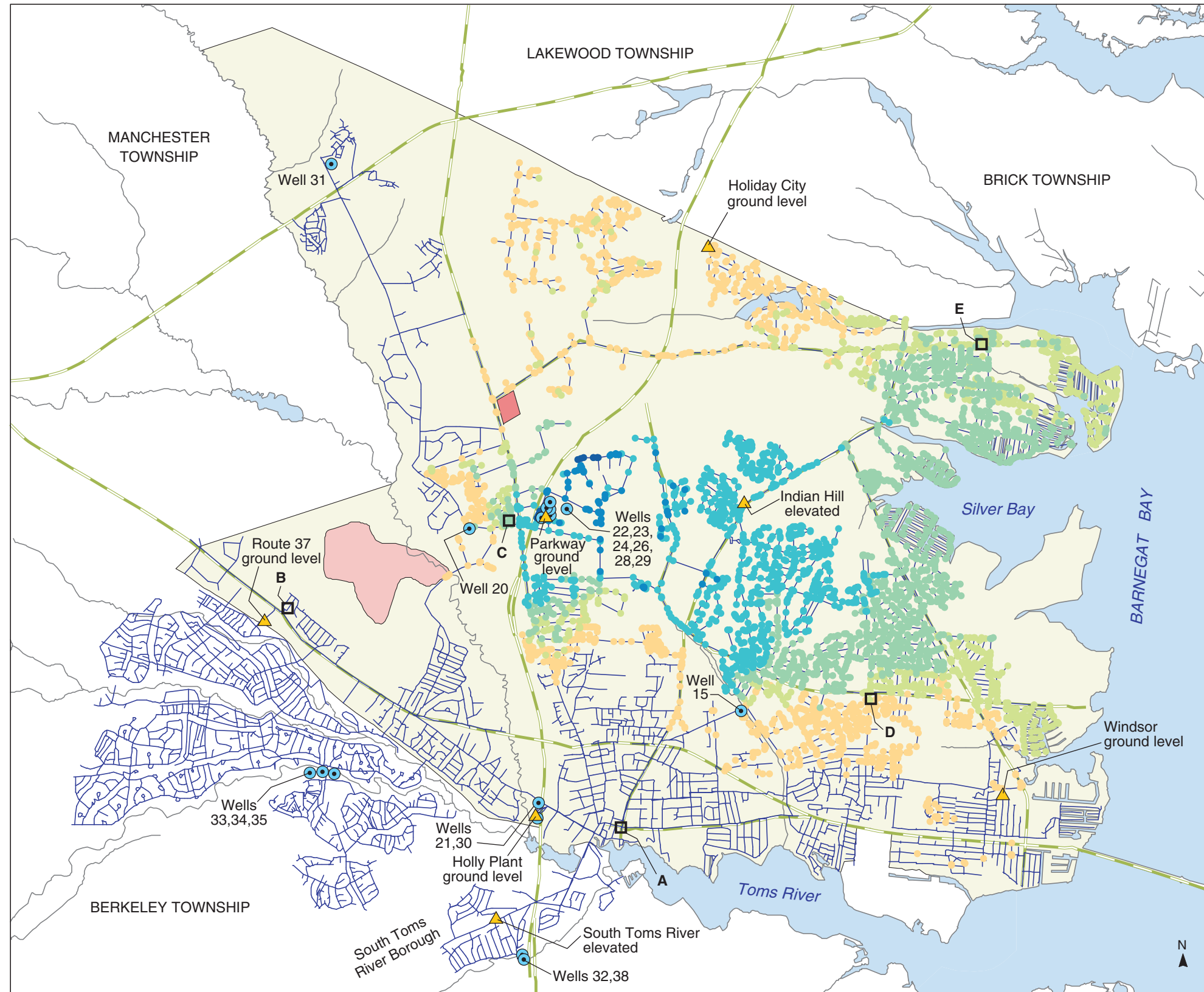
PLATE 102. AREAL DISTRIBUTION OF SIMULATED PROPORTIONATE CONTRIBUTION OF WATER FROM THE PARKWAY WELLS (22, 24) TO LOCATIONS IN THE DOVER TOWNSHIP AREA, NEW JERSEY, FEBRUARY 1988 CONDITIONS By Morris L. Maslia, Jason B. Sautner, Mustafa M. Aral, Richard E. Gillig, Juan J. Reyes, and Robert C. Williams
