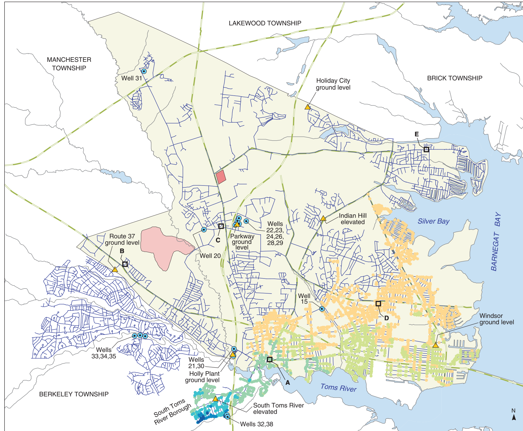
PLATE 101. AREAL DISTRIBUTION OF SIMULATED PROPORTIONATE CONTRIBUTION OF WATER FROM THE SOUTH TOMS RIVER WELL (32) TO LOCATIONS IN THE DOVER TOWNSHIP AREA, NEW JERSEY, FEBRUARY 1988 CONDITIONS
