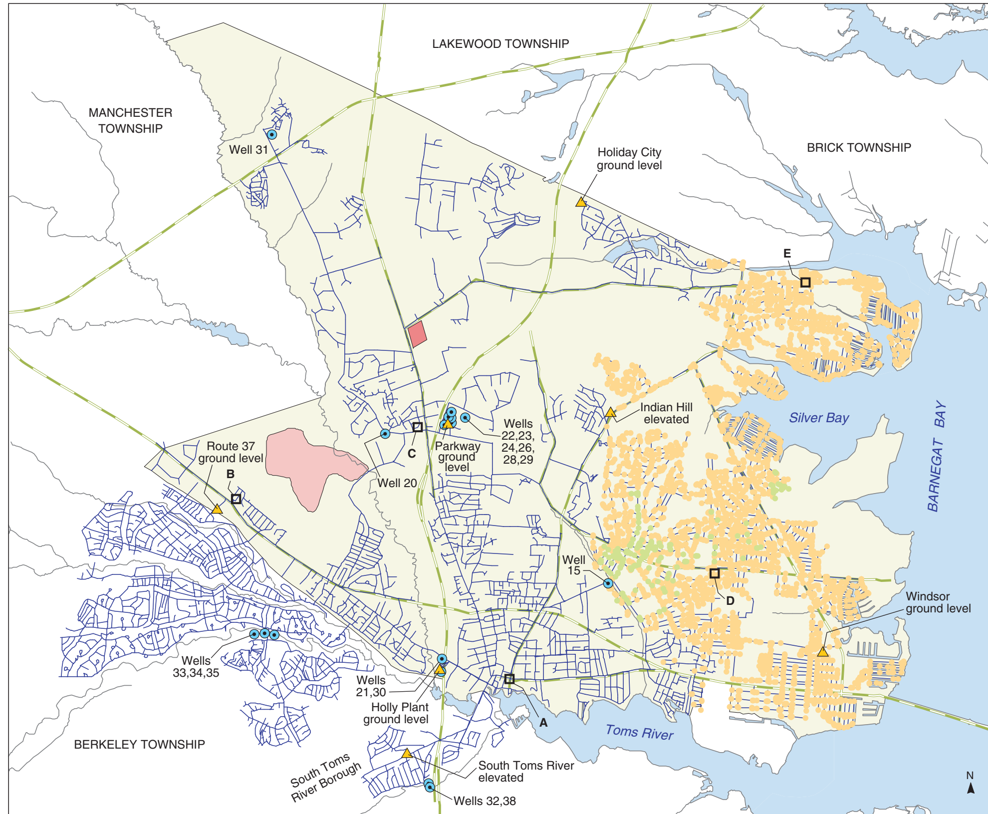
PLATE 100. AREAL DISTRIBUTION OF SIMULATED PROPORTIONATE CONTRIBUTION OF WATER FROM THE BROOKSIDE WELL (15) TO LOCATIONS IN THE DOVER TOWNSHIP AREA, NEW JERSEY, FEBRUARY 1988 CONDITIONS By Morris L. Maslia, Jason B. Sautner, Mustafa M. Aral, Richard E. Gillig, Juan J. Reyes, and Robert C. Williams
