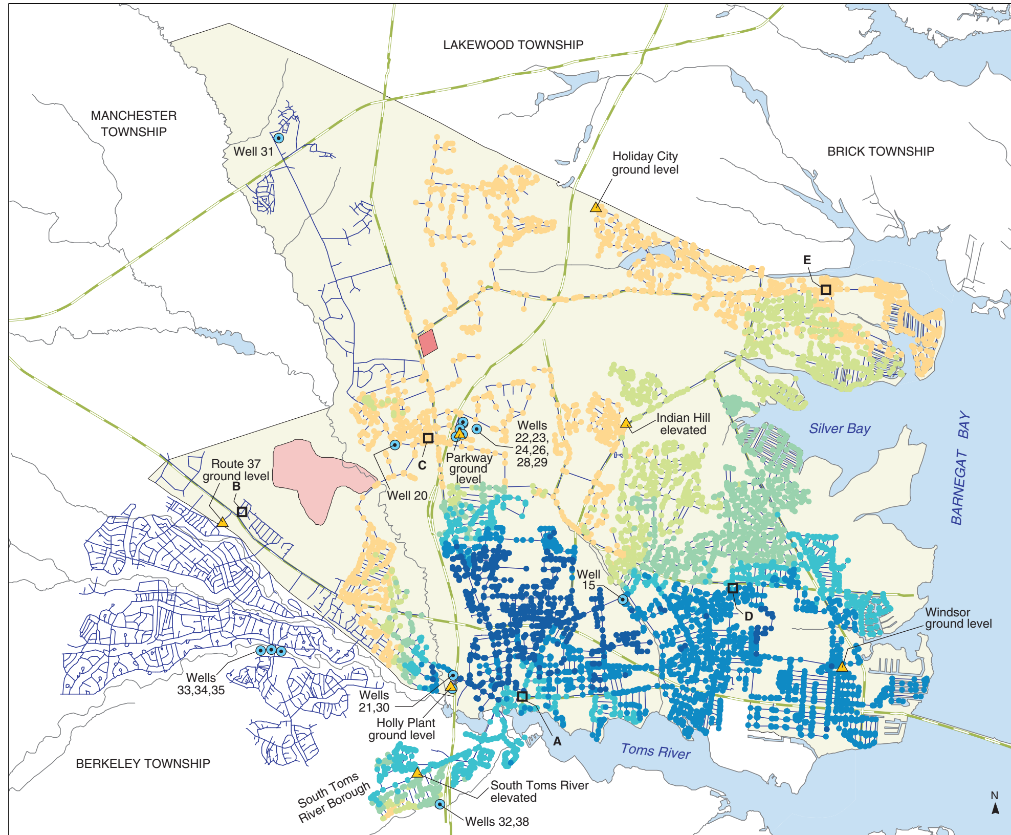
PLATE 99. AREAL DISTRIBUTION OF SIMULATED PROPORTIONATE CONTRIBUTION OF WATER FROM THE HOLLY WELL (30) TO LOCATIONS IN THE DOVER TOWNSHIP AREA, NEW JERSEY, FEBRUARY 1988 CONDITIONS
