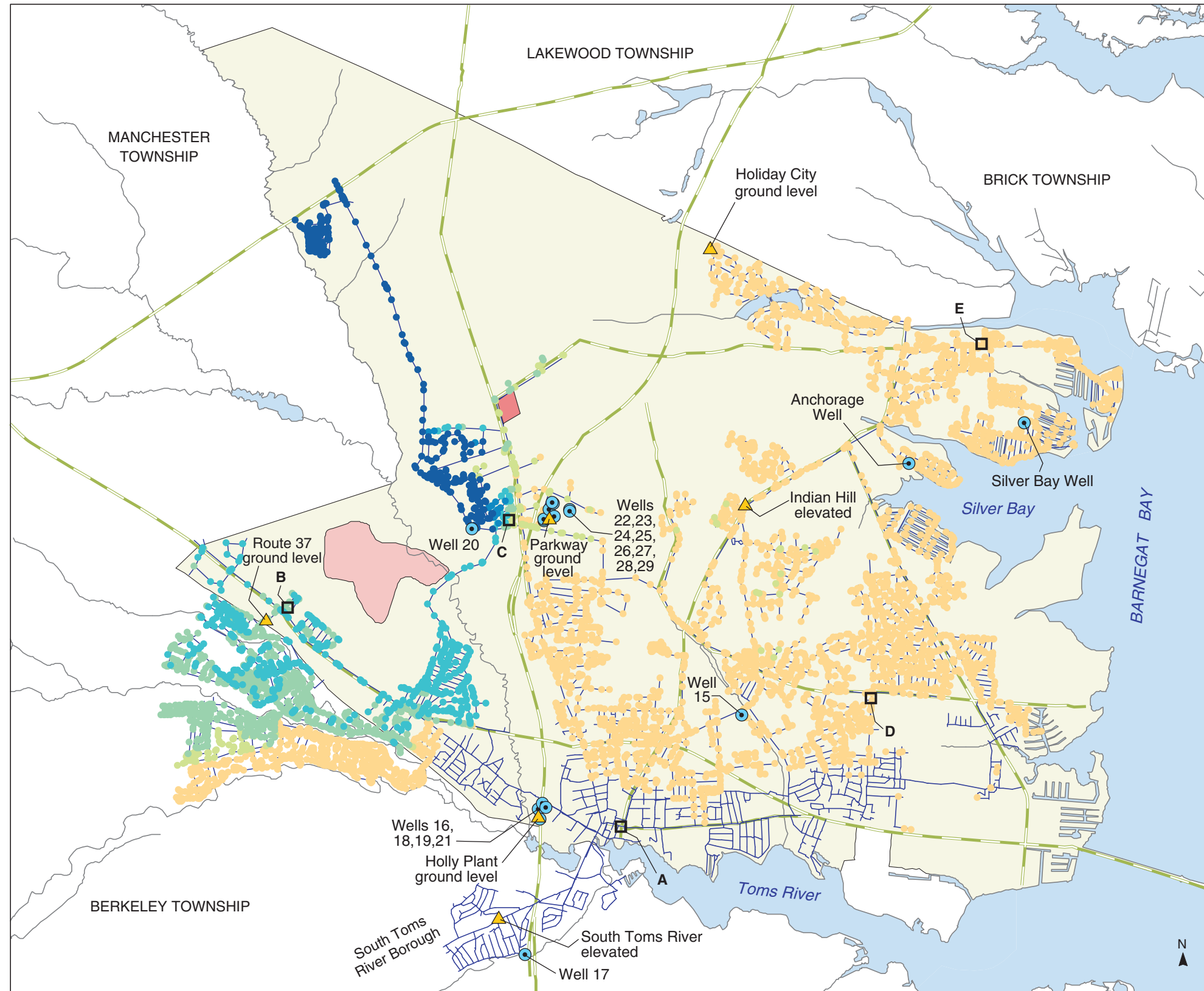
PLATE 97. AREAL DISTRIBUTION OF SIMULATED PROPORTIONATE CONTRIBUTION OF WATER FROM THE INDIAN HEAD WELL (20) TO LOCATIONS IN THE DOVER TOWNSHIP AREA, NEW JERSEY, OCTOBER 1978 CONDITIONS By Morris L. Maslia, Jason B. Sautner, Mustafa M. Aral, Richard E. Gillig, Juan J. Reyes, and Robert C. Williams
