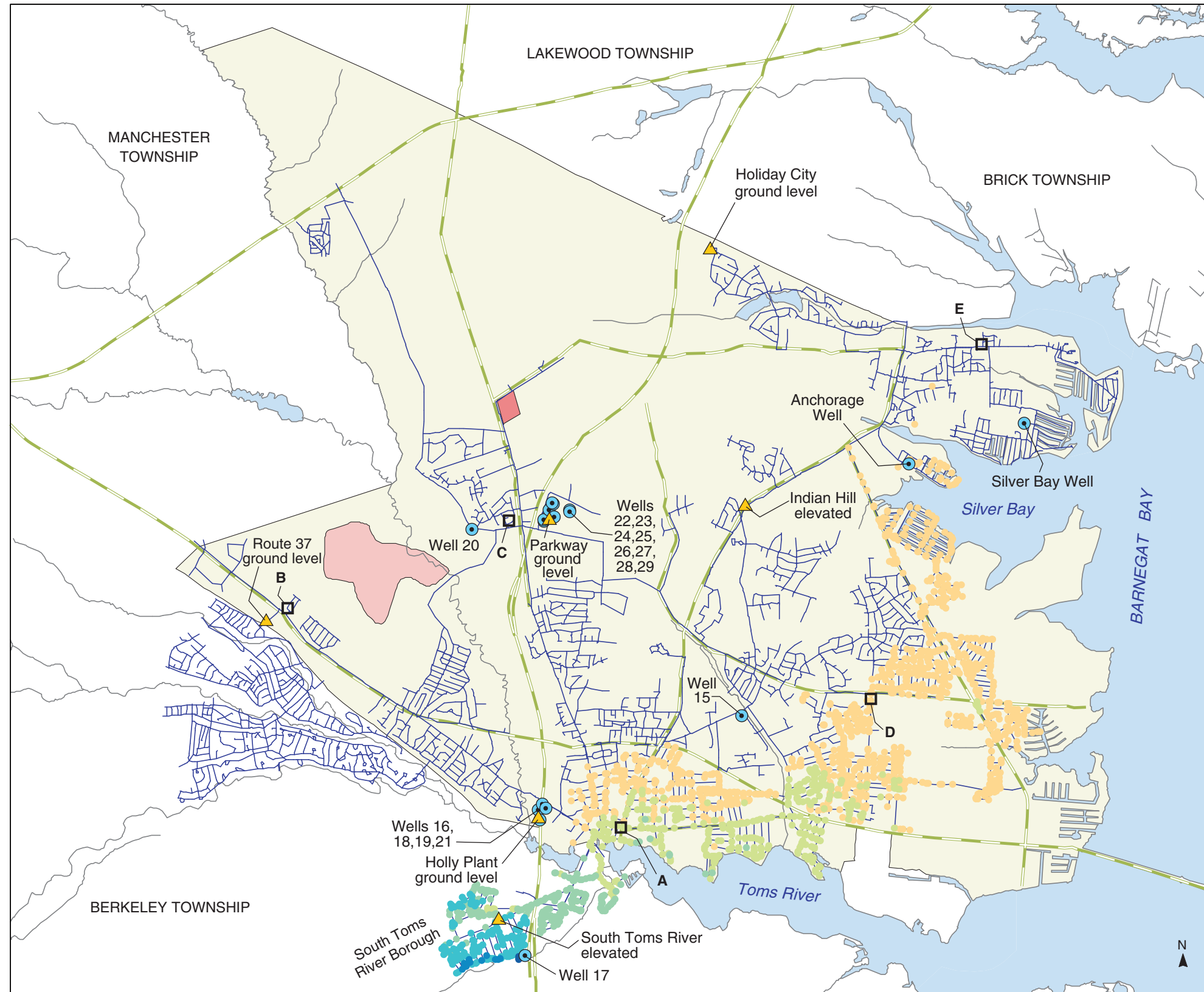
PLATE 96. AREAL DISTRIBUTION OF SIMULATED PROPORTIONATE CONTRIBUTION OF WATER FROM THE SOUTH TOMS RIVER WELL (17) TO LOCATIONS IN THE DOVER TOWNSHIP AREA, NEW JERSEY, OCTOBER 1978 CONDITIONS
