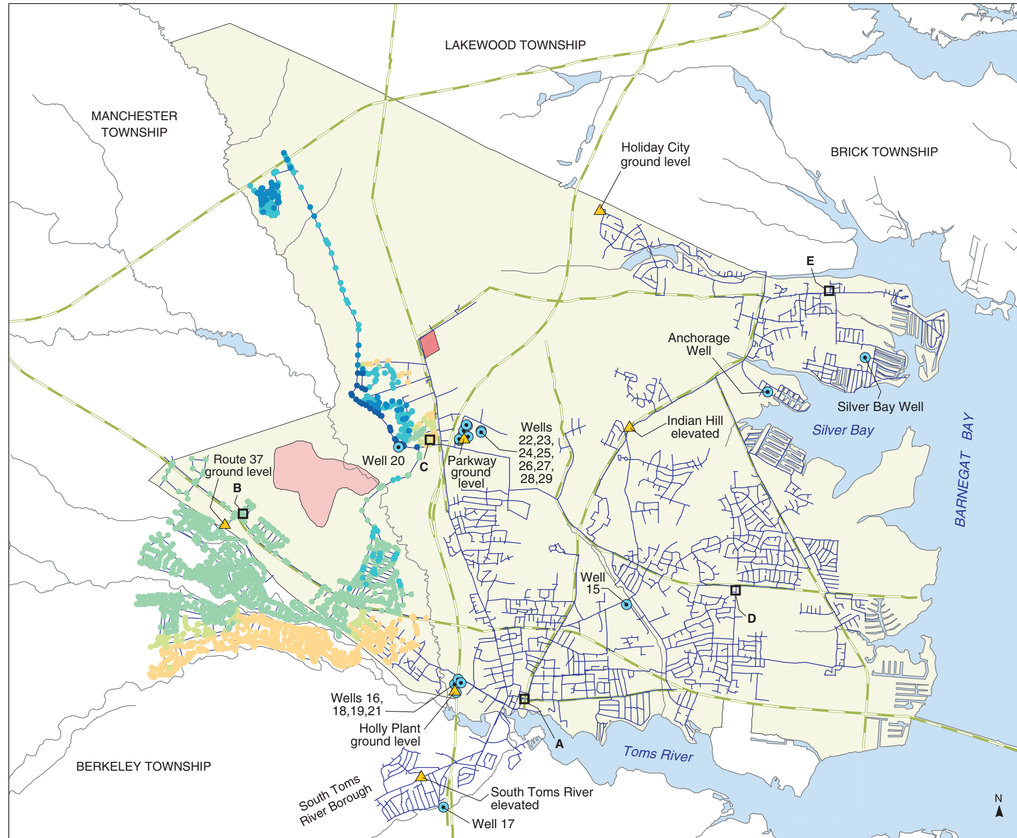
PLATE 90. AREAL DISTRIBUTION OF SIMULATED PROPORTIONATE CONTRIBUTION OF WATER FROM THE INDIAN HEAD WELL (20) TO LOCATIONS IN THE DOVER TOWNSHIP AREA, NEW JERSEY, JUNE 1978 CONDITIONS
