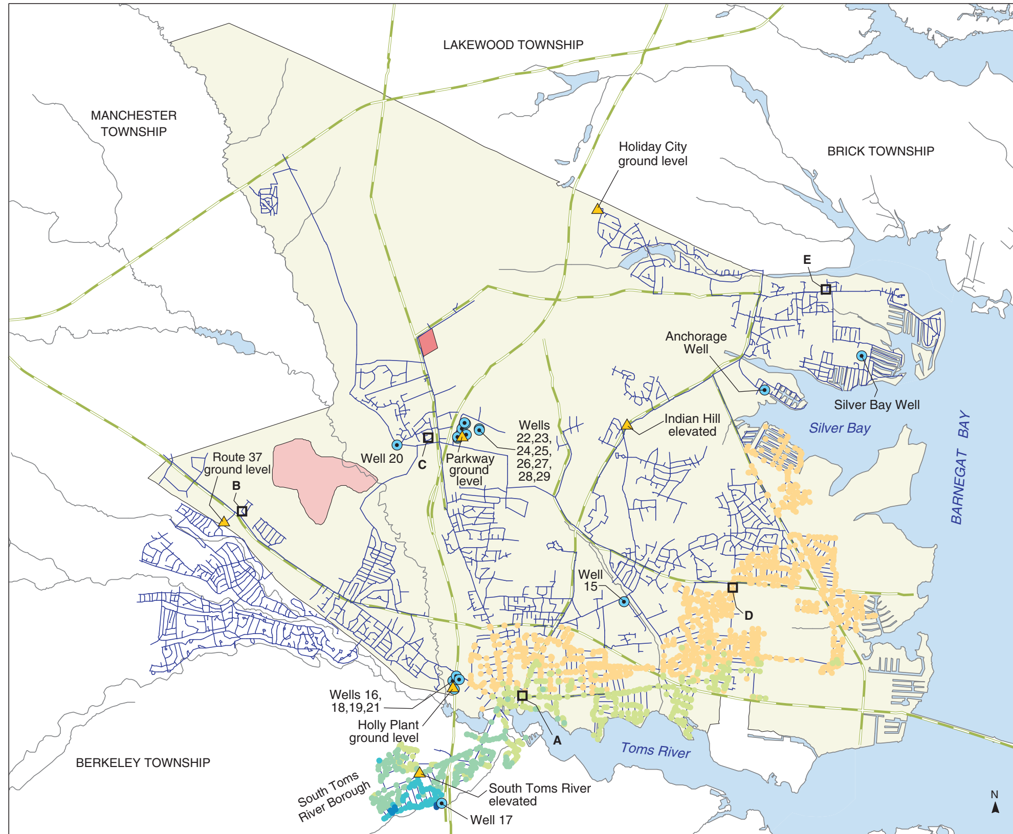
PLATE 89. AREAL DISTRIBUTION OF SIMULATED PROPORTIONATE CONTRIBUTION OF WATER FROM THE SOUTH TOMS RIVER WELL (17) TO LOCATIONS IN THE DOVER TOWNSHIP AREA, NEW JERSEY, JUNE 1978 CONDITIONS
