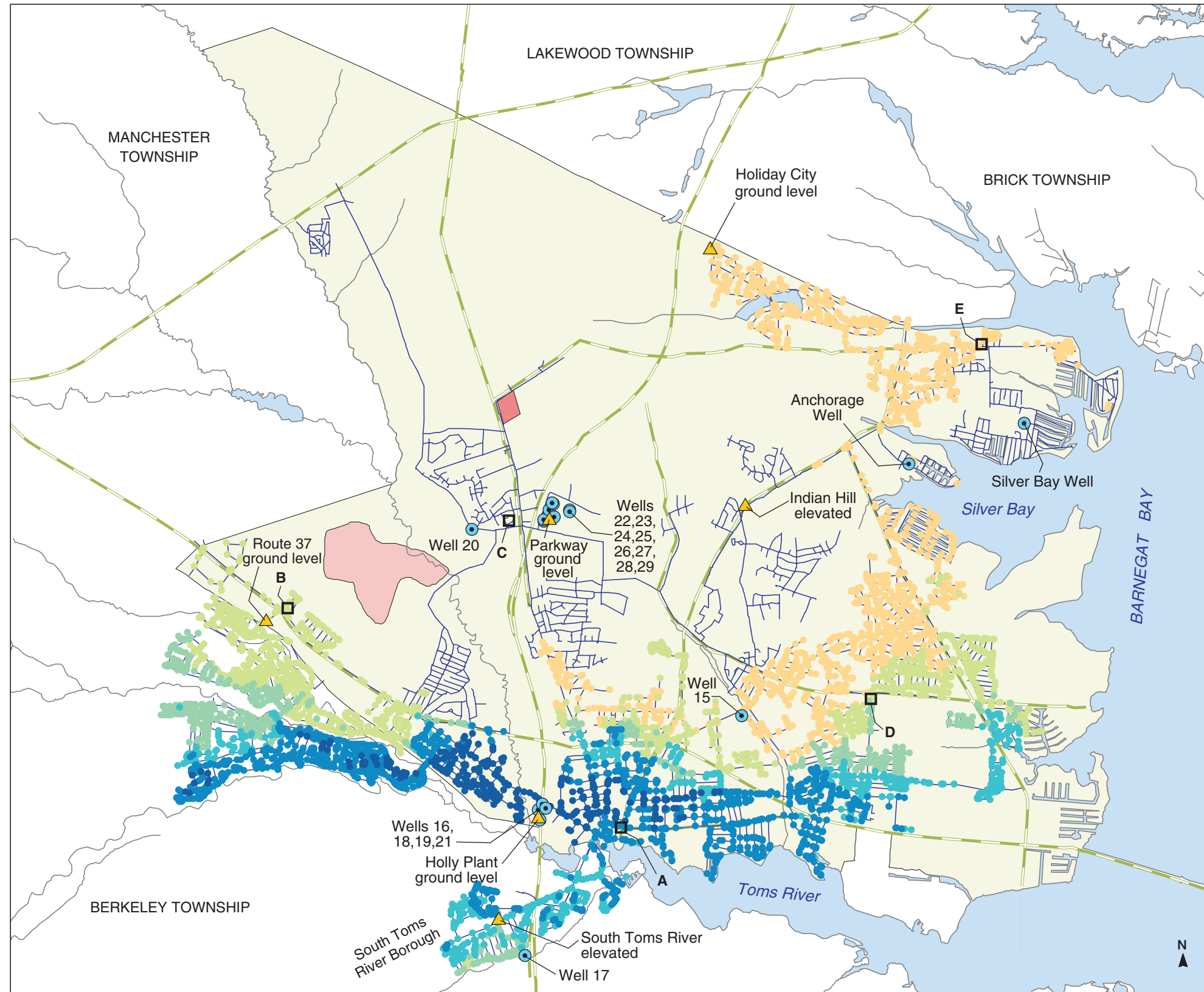
PLATE 87. AREAL DISTRIBUTION OF SIMULATED PROPORTIONATE CONTRIBUTION OF WATER FROM THE HOLLY WELLS (16, 18, 19, 21) TO LOCATIONS IN THE DOVER TOWNSHIP AREA, NEW JERSEY, JUNE 1978 CONDITIONS By Morris L. Maslia, Jason B. Sautner, Mustafa M. Aral, Richard E. Gillig, Juan J. Reyes, and Robert C. Williams
