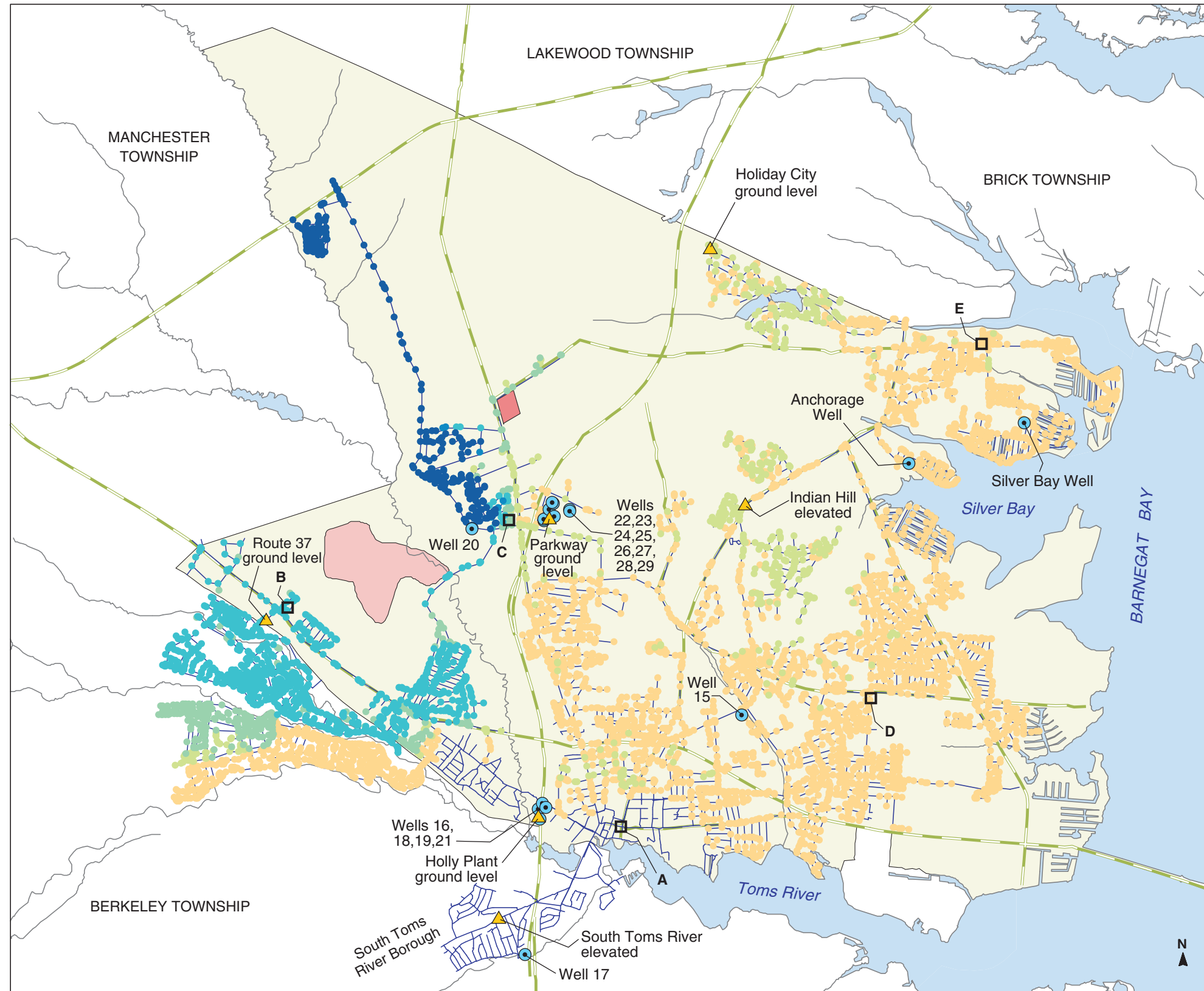
PLATE 85. AREAL DISTRIBUTION OF SIMULATED PROPORTIONATE CONTRIBUTION OF WATER FROM THE INDIAN HEAD WELL (20) TO LOCATIONS IN THE DOVER TOWNSHIP AREA, NEW JERSEY, FEBRUARY 1978 CONDITIONS
