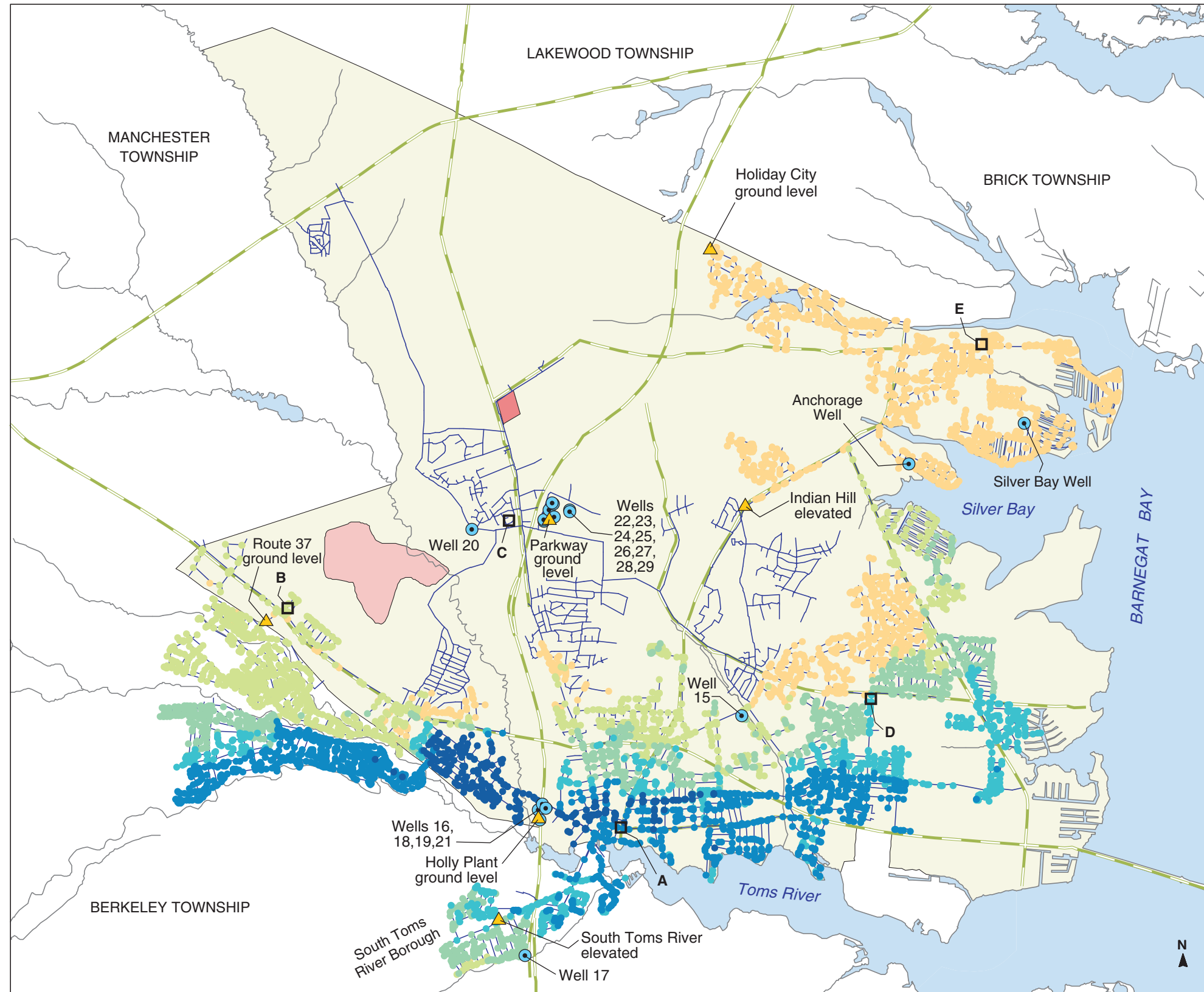
PLATE 83. AREAL DISTRIBUTION OF SIMULATED PROPORTIONATE CONTRIBUTION OF WATER FROM THE HOLLY WELLS (16, 18) TO LOCATIONS IN THE DOVER TOWNSHIP AREA, NEW JERSEY, FEBRUARY 1978 CONDITIONS By Morris L. Maslia, Jason B. Sautner, Mustafa M. Aral, Richard E. Gillig, Juan J. Reyes, and Robert C. Williams
