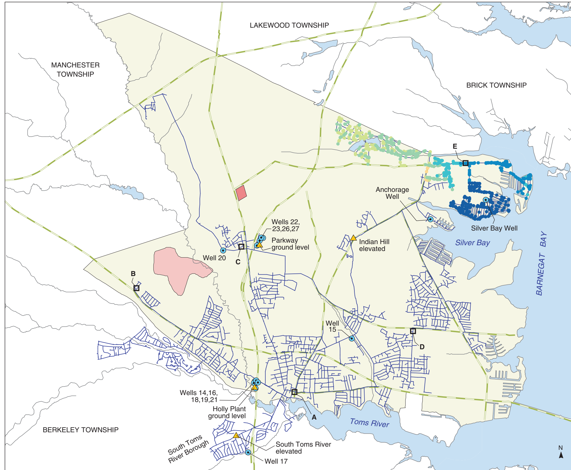
PLATE 82. AREAL DISTRIBUTION OF SIMULATED PROPORTIONATE CONTRIBUTION OF WATER FROM THE SILVER BAY WELL TO LOCATIONS IN THE DOVER TOWNSHIP AREA, NEW JERSEY, OCTOBER 1971 CONDITIONS
