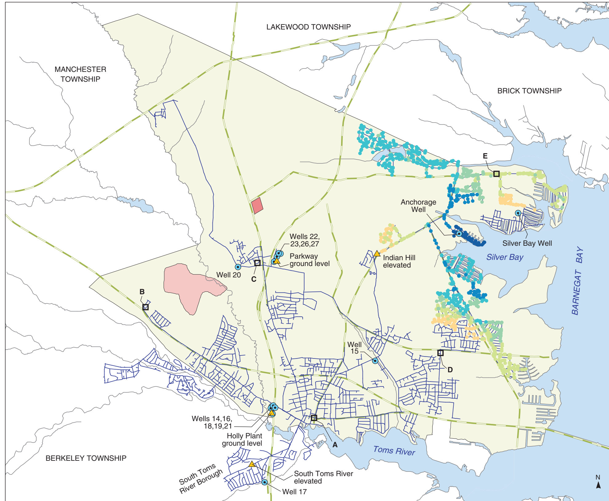
PLATE 81. AREAL DISTRIBUTION OF SIMULATED PROPORTIONATE CONTRIBUTION OF WATER FROM THE ANCHORAGE WELL TO LOCATIONS IN THE DOVER TOWNSHIP AREA, NEW JERSEY, OCTOBER 1971 CONDITIONS
