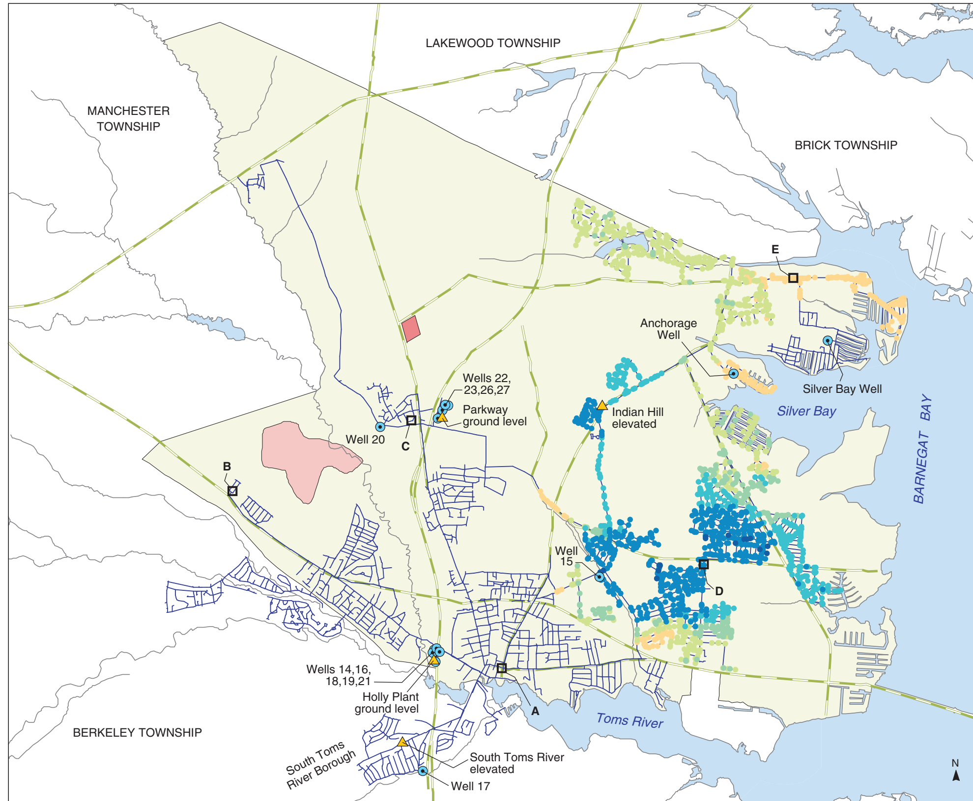
PLATE 78. AREAL DISTRIBUTION OF SIMULATED PROPORTIONATE CONTRIBUTION OF WATER FROM THE BROOKSIDE WELL (15) TO LOCATIONS IN THE DOVER TOWNSHIP AREA, NEW JERSEY, OCTOBER 1971 CONDITIONS By Morris L. Maslia, Jason B. Sautner, Mustafa M. Aral, Richard E. Gillig, Juan J. Reyes, and Robert C. Williams
