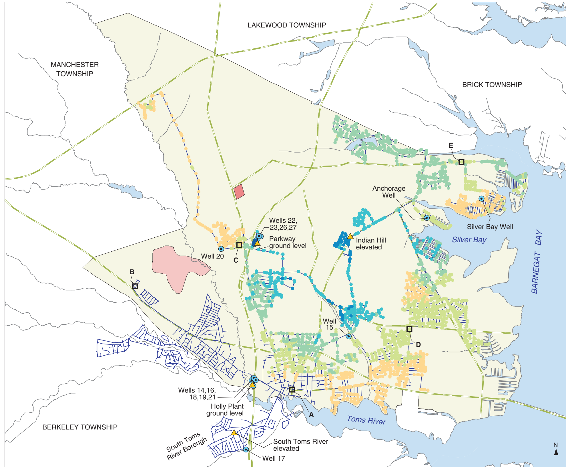
PLATE 74. AREAL DISTRIBUTION OF SIMULATED PROPORTIONATE CONTRIBUTION OF WATER FROM THE PARKWAY WELLS (22, 23, 26, 27) TO LOCATIONS IN THE DOVER TOWNSHIP AREA, NEW JERSEY, JULY 1971 CONDITIONS By Morris L. Maslia, Jason B. Sautner, Mustafa M. Aral, Richard E. Gillig, Juan J. Reyes, and Robert C. Williams
