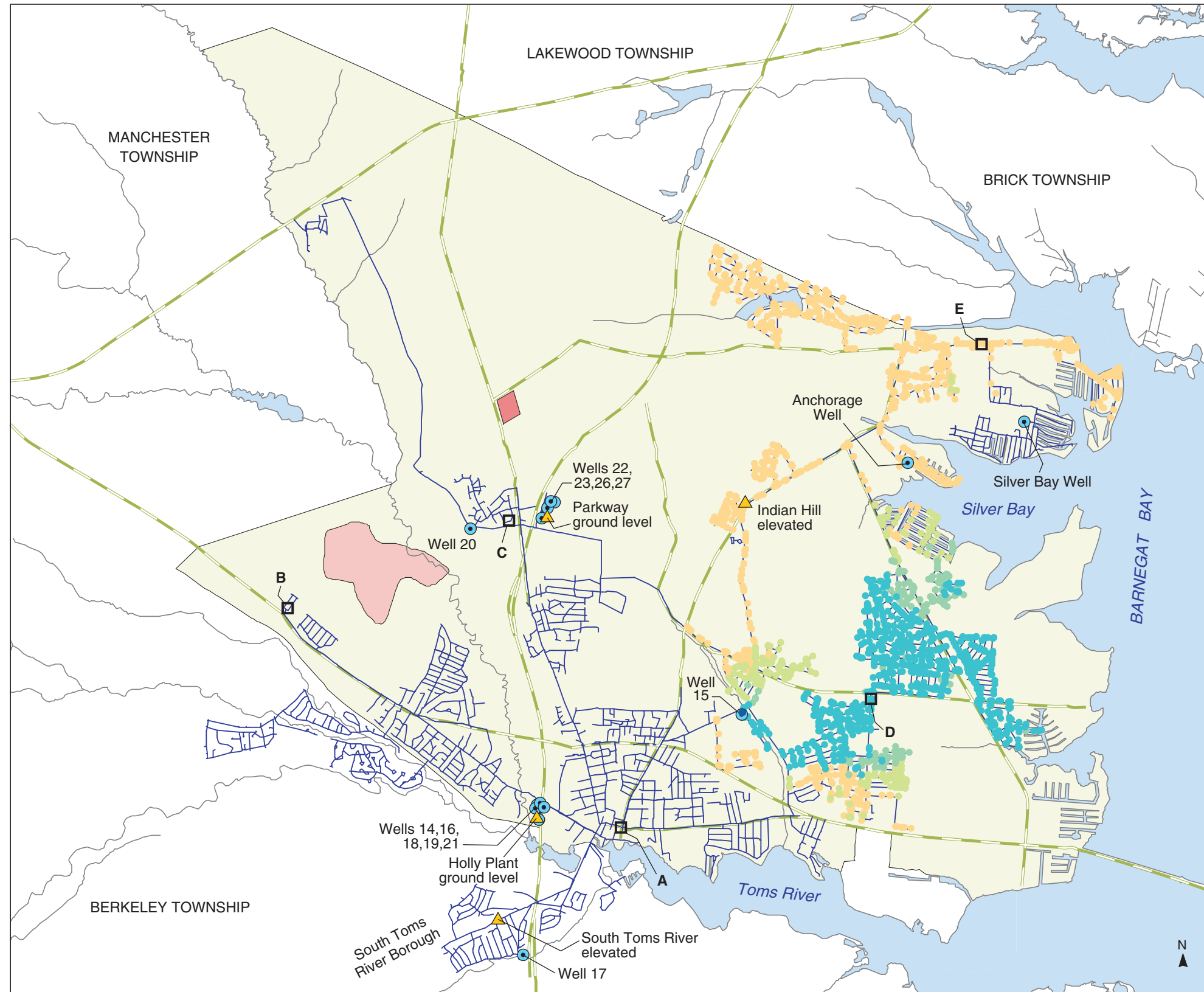
PLATE 71. AREAL DISTRIBUTION OF SIMULATED PROPORTIONATE CONTRIBUTION OF WATER FROM THE BROOKSIDE WELL (15) TO LOCATIONS IN THE DOVER TOWNSHIP AREA, NEW JERSEY, JULY 1971 CONDITIONS
