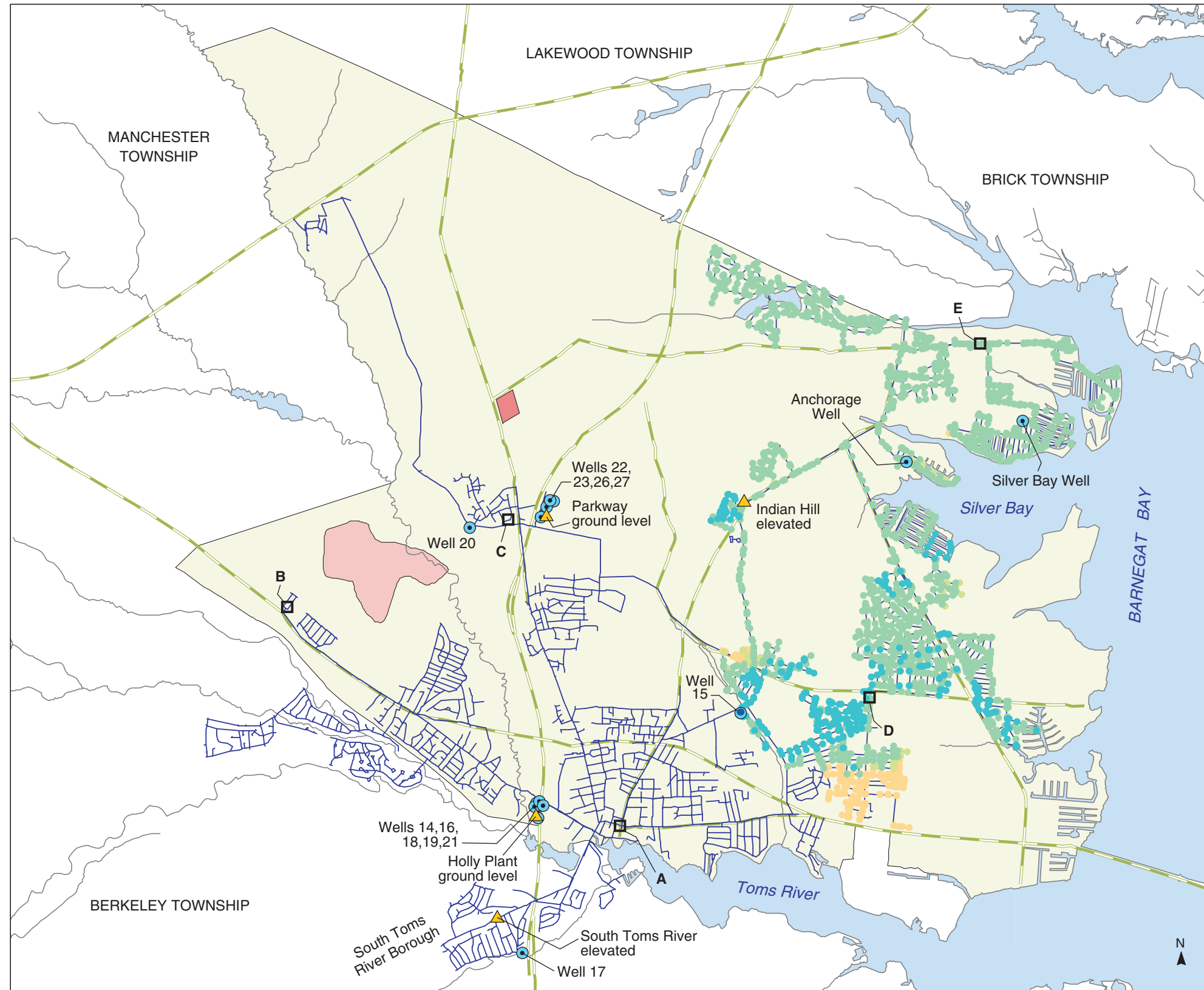
PLATE 65. AREAL DISTRIBUTION OF SIMULATED PROPORTIONATE CONTRIBUTION OF WATER FROM THE BROOKSIDE WELL (15) TO LOCATIONS IN THE DOVER TOWNSHIP AREA, NEW JERSEY, FEBRUARY 1971 CONDITIONS By Morris L. Maslia, Jason B. Sautner, Mustafa M. Aral, Richard E. Gillig, Juan J. Reyes, and Robert C. Williams
