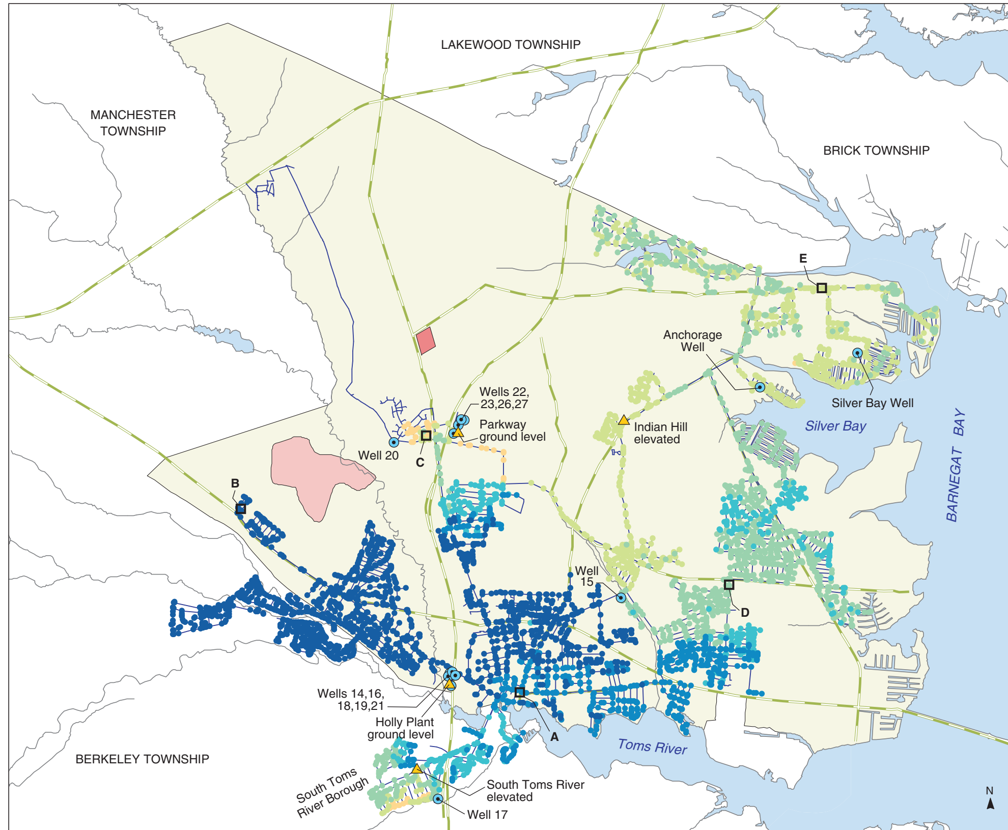
PLATE 64. AREAL DISTRIBUTION OF SIMULATED PROPORTIONATE CONTRIBUTION OF WATER FROM THE HOLLY WELLS (16, 18, 19) TO LOCATIONS IN THE DOVER TOWNSHIP AREA, NEW JERSEY, FEBRUARY 1971 CONDITIONS By Morris L. Maslia, Jason B. Sautner, Mustafa M. Aral, Richard E. Gillig, Juan J. Reyes, and Robert C. Williams
