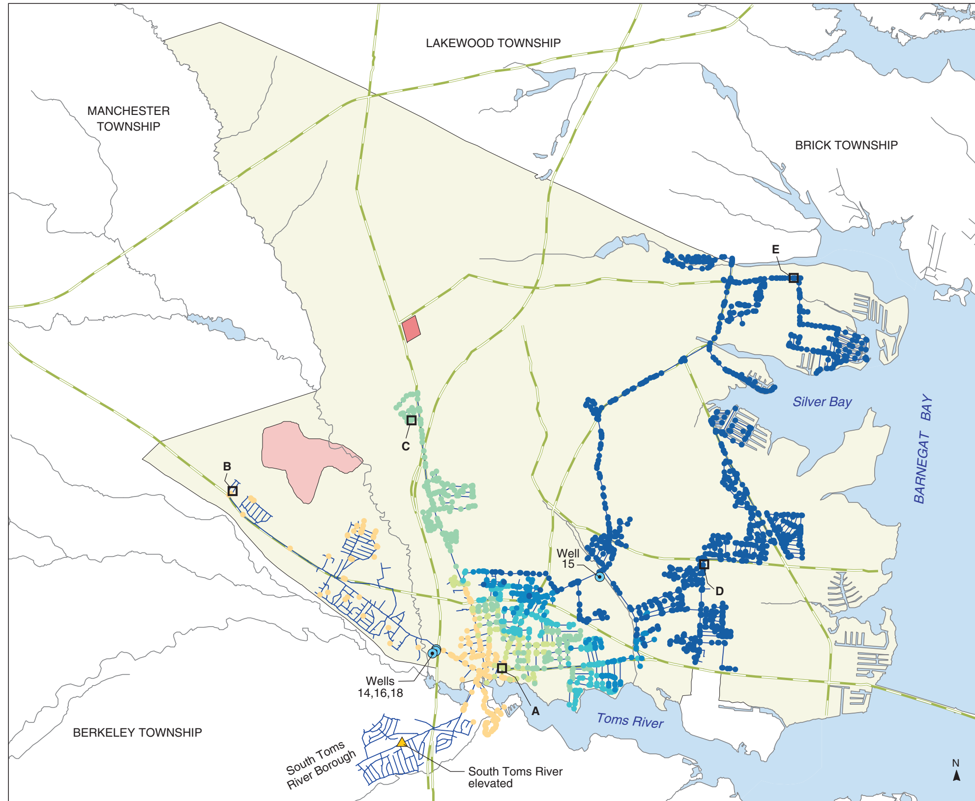
PLATE 63. AREAL DISTRIBUTION OF SIMULATED PROPORTIONATE CONTRIBUTION OF WATER FROM THE BROOKSIDE WELL (15) TO LOCATIONS IN THE DOVER TOWNSHIP AREA, NEW JERSEY, OCTOBER 1965 CONDITIONS
