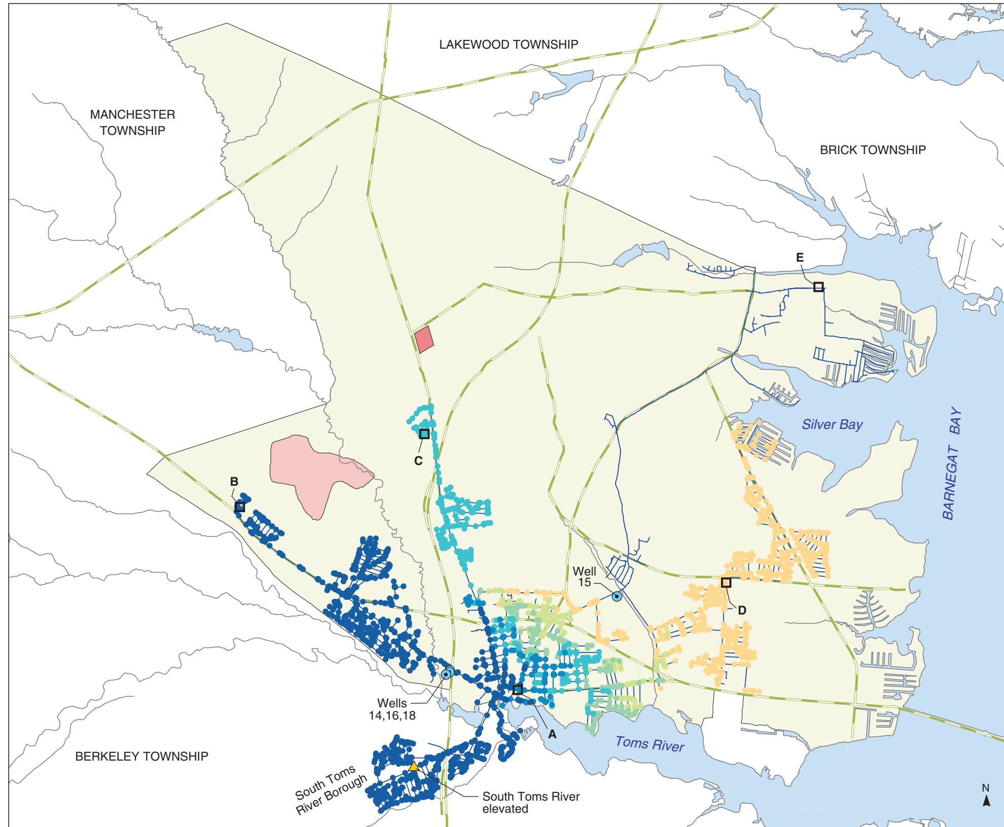
PLATE 62. AREAL DISTRIBUTION OF SIMULATED PROPORTIONATE CONTRIBUTION OF WATER FROM THE HOLLY WELLS (14, 16, 18) TO LOCATIONS IN THE DOVER TOWNSHIP AREA, NEW JERSEY, OCTOBER 1965 CONDITIONS By Morris L. Maslia, Jason B. Sautner, Mustafa M. Aral, Richard E. Gillig, Juan J. Reyes, and Robert C. Williams
