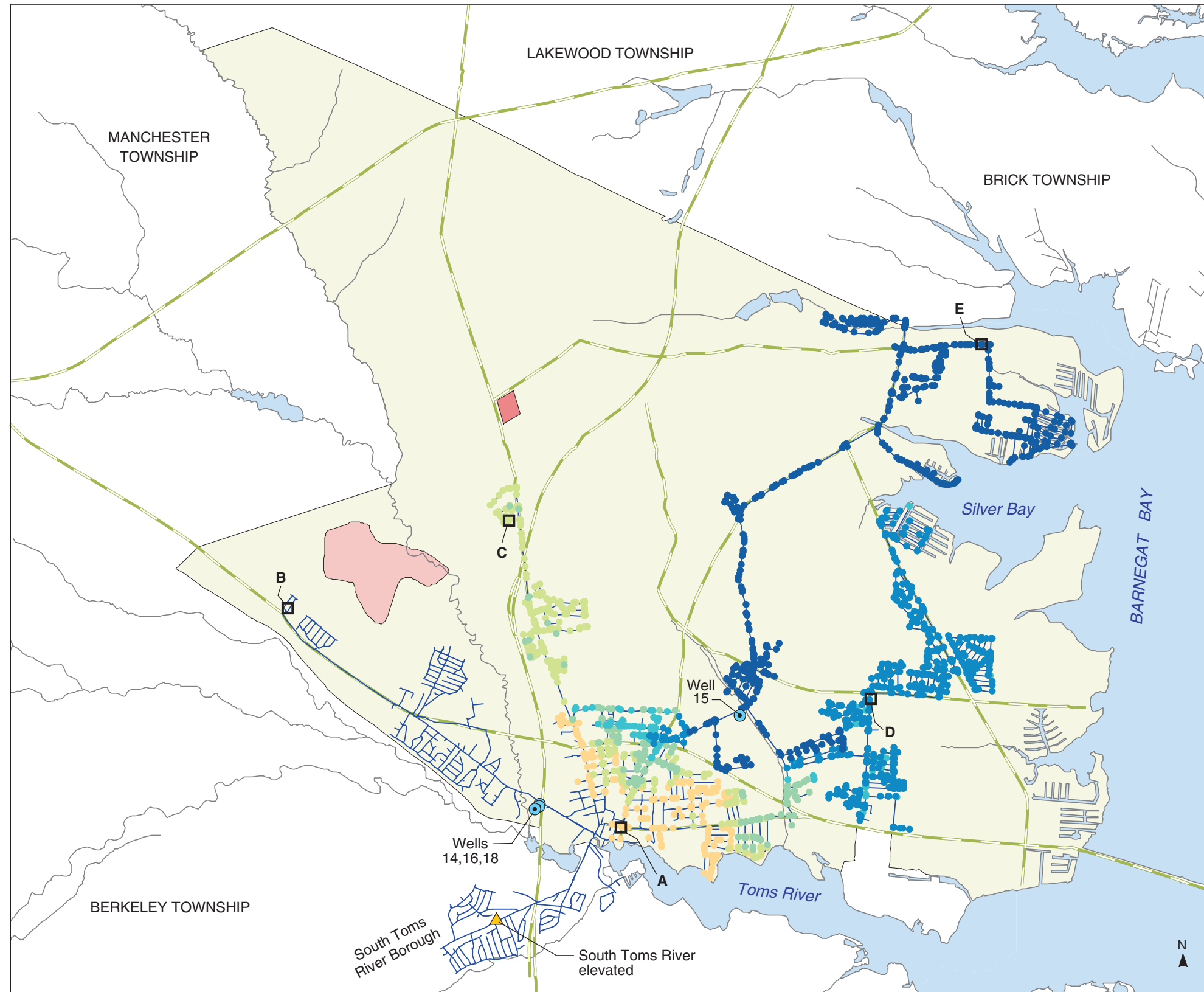
PLATE 61. AREAL DISTRIBUTION OF SIMULATED PROPORTIONATE CONTRIBUTION OF WATER FROM THE BROOKSIDE WELL (15) TO LOCATIONS IN THE DOVER TOWNSHIP AREA, NEW JERSEY, JUNE 1965 CONDITIONS
