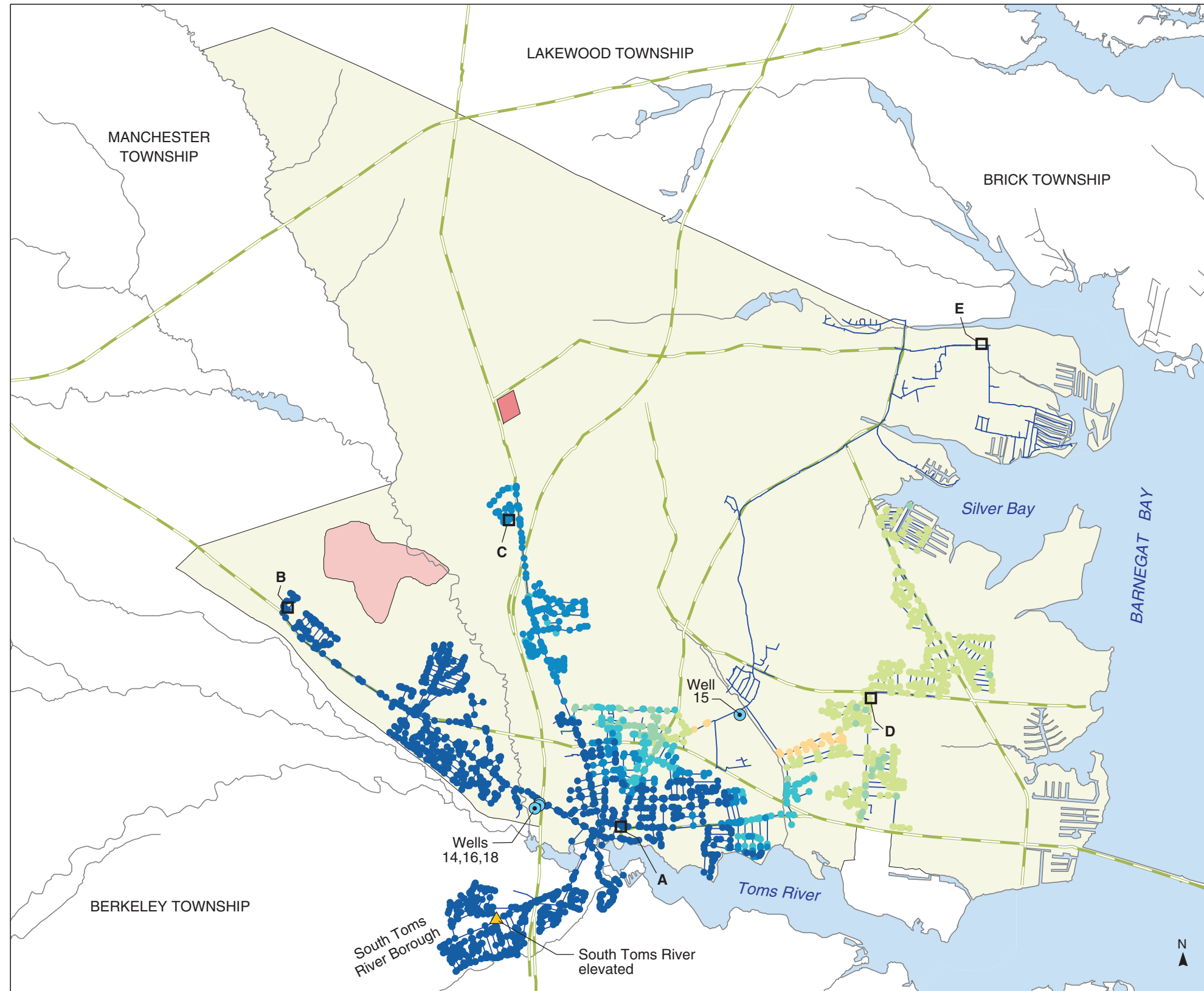
PLATE 60. AREAL DISTRIBUTION OF SIMULATED PROPORTIONATE CONTRIBUTION OF WATER FROM THE HOLLY WELLS (14, 16, 18) TO LOCATIONS IN THE DOVER TOWNSHIP AREA, NEW JERSEY, JUNE 1965 CONDITIONS
