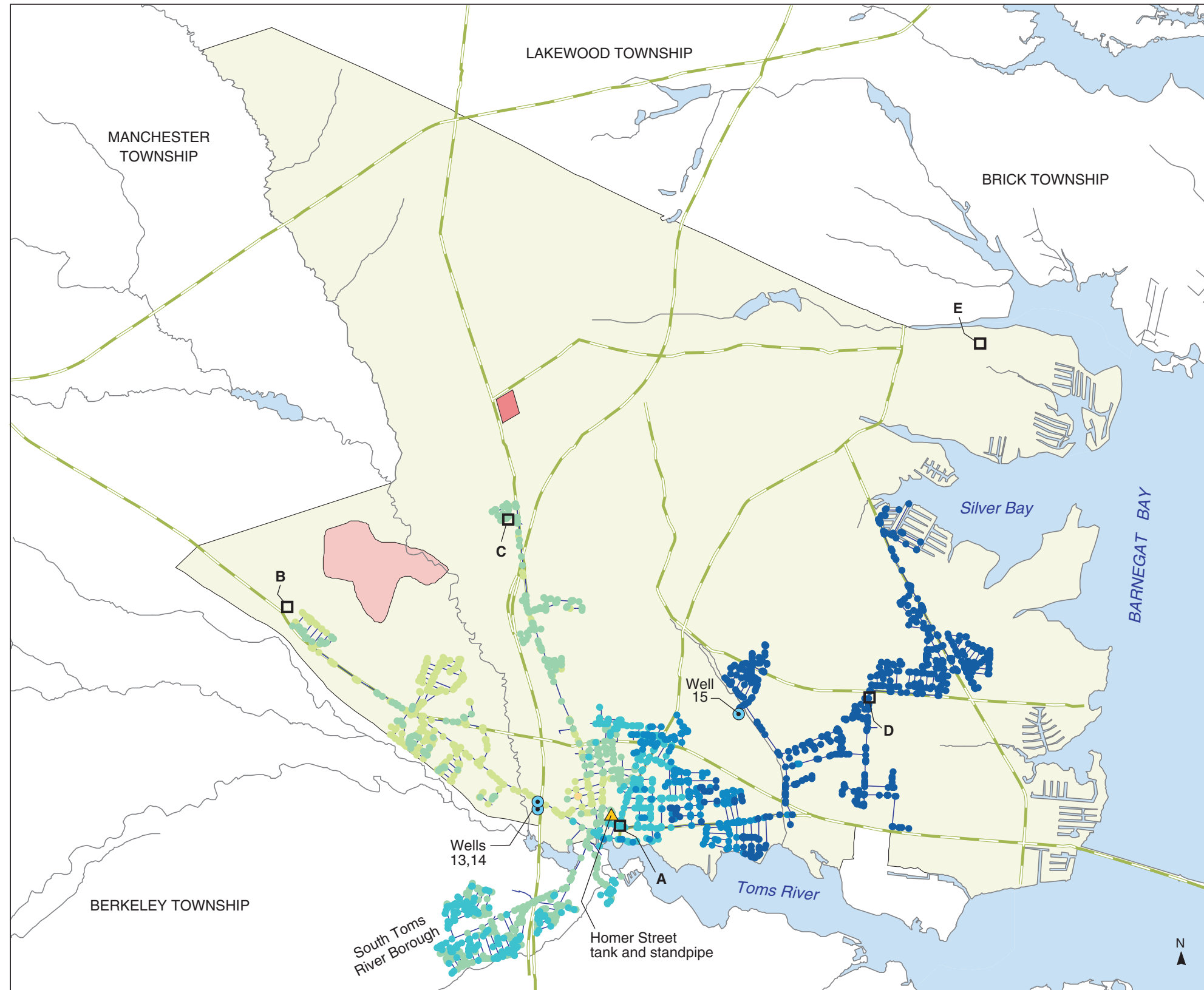
PLATE 57. AREAL DISTRIBUTION OF SIMULATED PROPORTIONATE CONTRIBUTION OF WATER FROM THE BROOKSIDE WELL (15) TO LOCATIONS IN THE DOVER TOWNSHIP AREA, NEW JERSEY, OCTOBER 1962 CONDITIONS By Morris L. Maslia, Jason B. Sautner, Mustafa M. Aral, Richard E. Gillig, Juan J. Reyes, and Robert C. Williams
