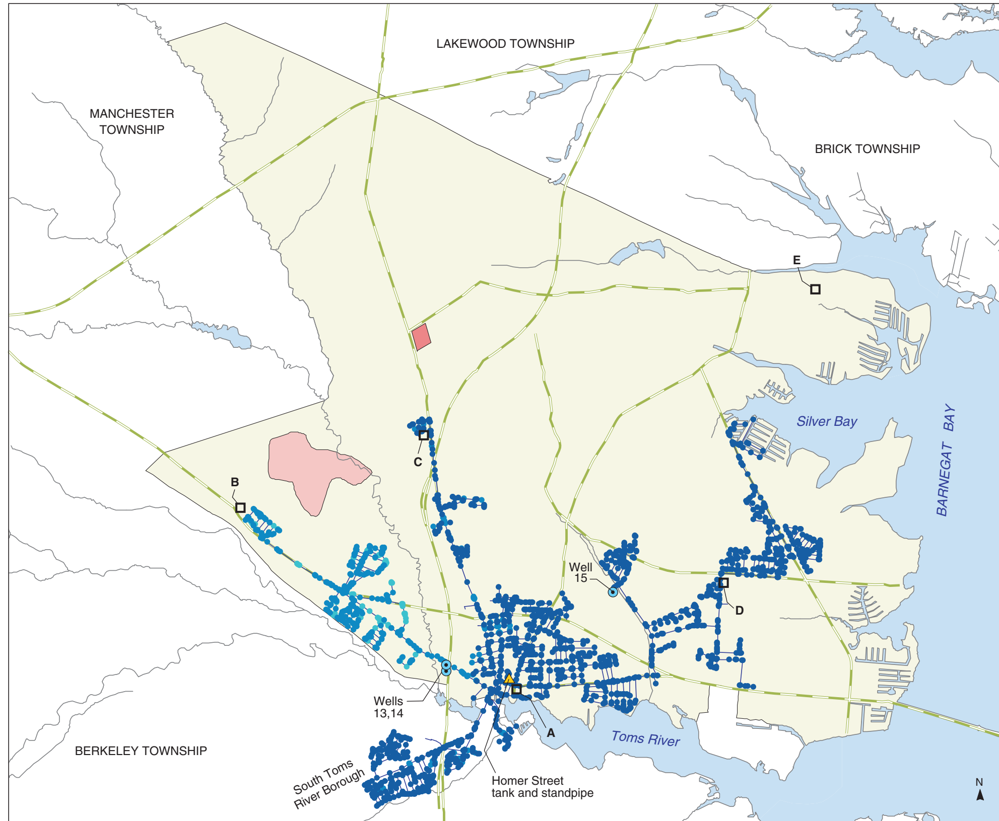
PLATE 53. AREAL DISTRIBUTION OF SIMULATED PROPORTIONATE CONTRIBUTION OF WATER FROM THE BROOKSIDE WELL (15) TO LOCATIONS IN THE DOVER TOWNSHIP AREA, NEW JERSEY, FEBRUARY 1962 CONDITIONS
