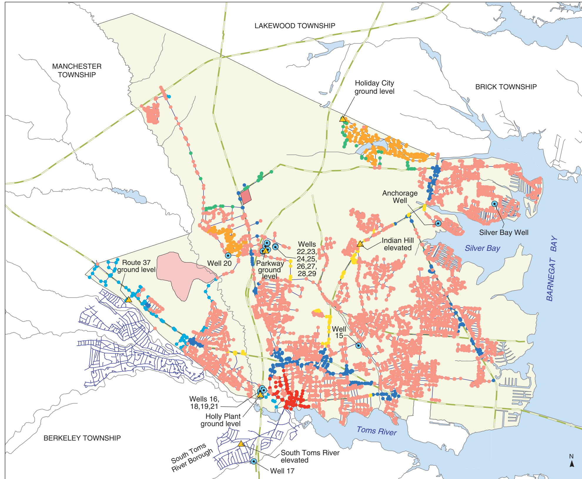
PLATE 49. AREAL DISTRIBUTION OF LAND-USE CLASSIFICATION ASSIGNED TO PIPELINE NODES 1978 WATER-DISTRIBUTION SYSTEM, DOVER TOWNSHIP AREA, NEW JERSEY By Morris L. Maslia, Jason B. Sautner, Mustafa M. Aral, Richard E. Gillig, Juan J. Reyes, and Robert C. Williams
