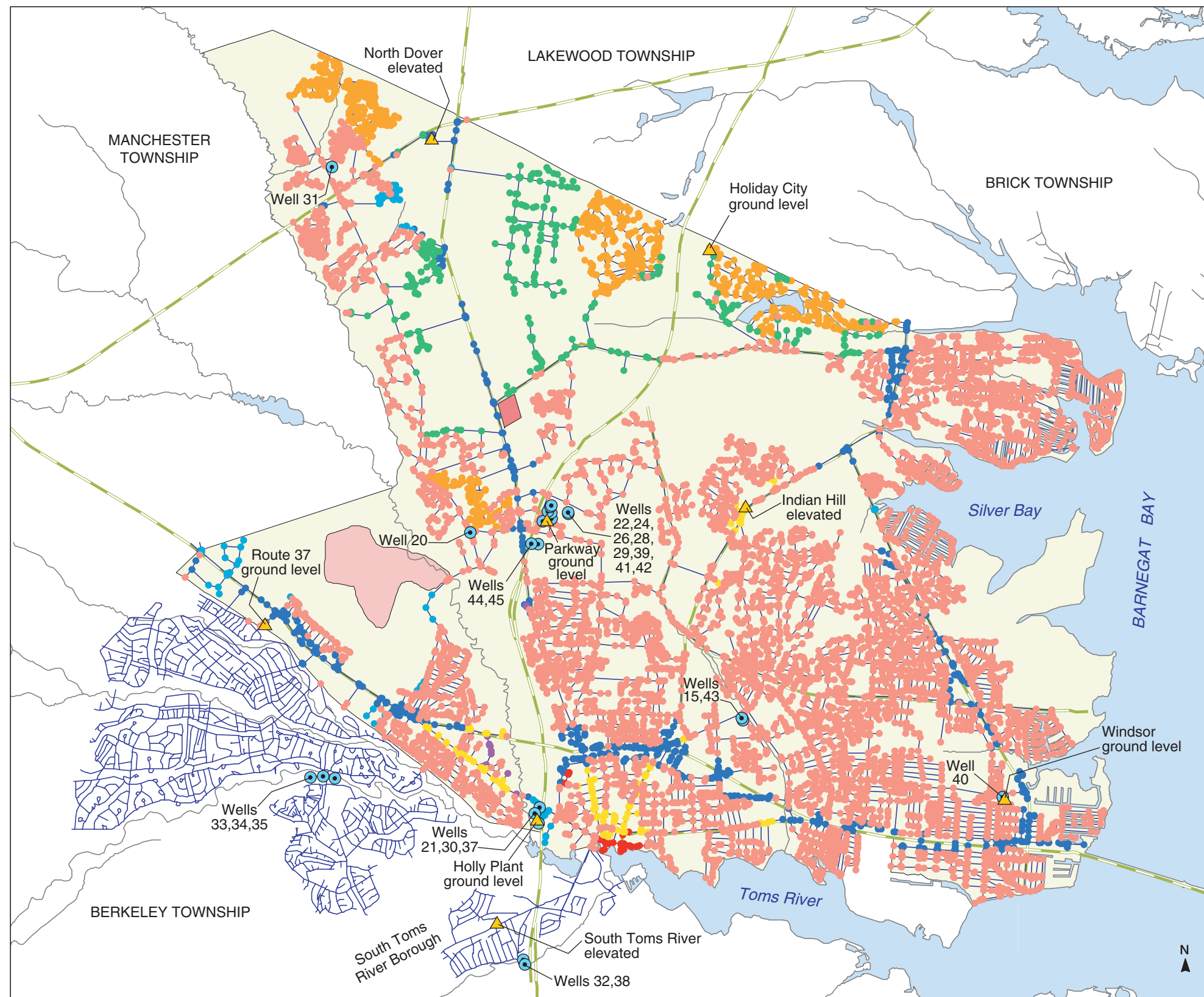
PLATE 46. AREAL DISTRIBUTION OF LAND-USE CLASSIFICATION ASSIGNED TO PIPELINE NODES 1998 WATER-DISTRIBUTION SYSTEM, DOVER TOWNSHIP AREA, NEW JERSEY By Morris L. Maslia, Jason B. Sautner, Mustafa M. Aral, Richard E. Gillig, Juan J. Reyes, and Robert C. Williams
