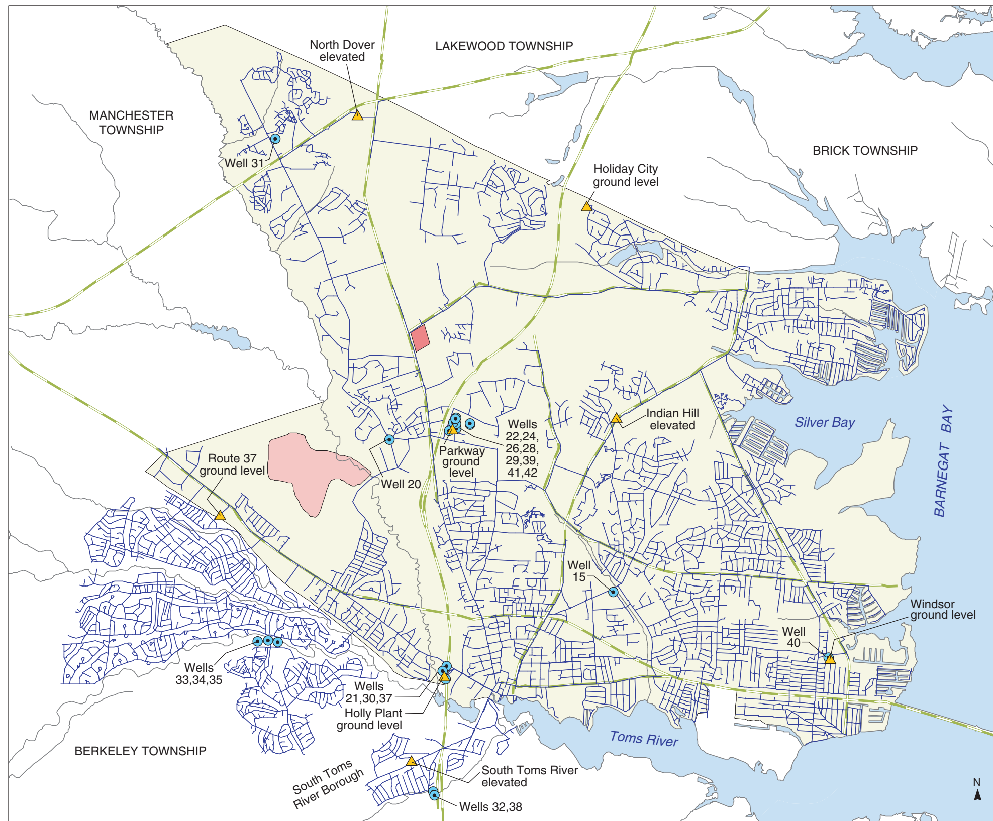
PLATE 37. WATER-DISTRIBUTION SYSTEM SERVING THE DOVER TOWNSHIP AREA, NEW JERSEY, 1996 By Morris L. Maslia, Jason B. Sautner, Mustafa M. Aral, Richard E. Gillig, Juan J. Reyes, and Robert C. Williams
