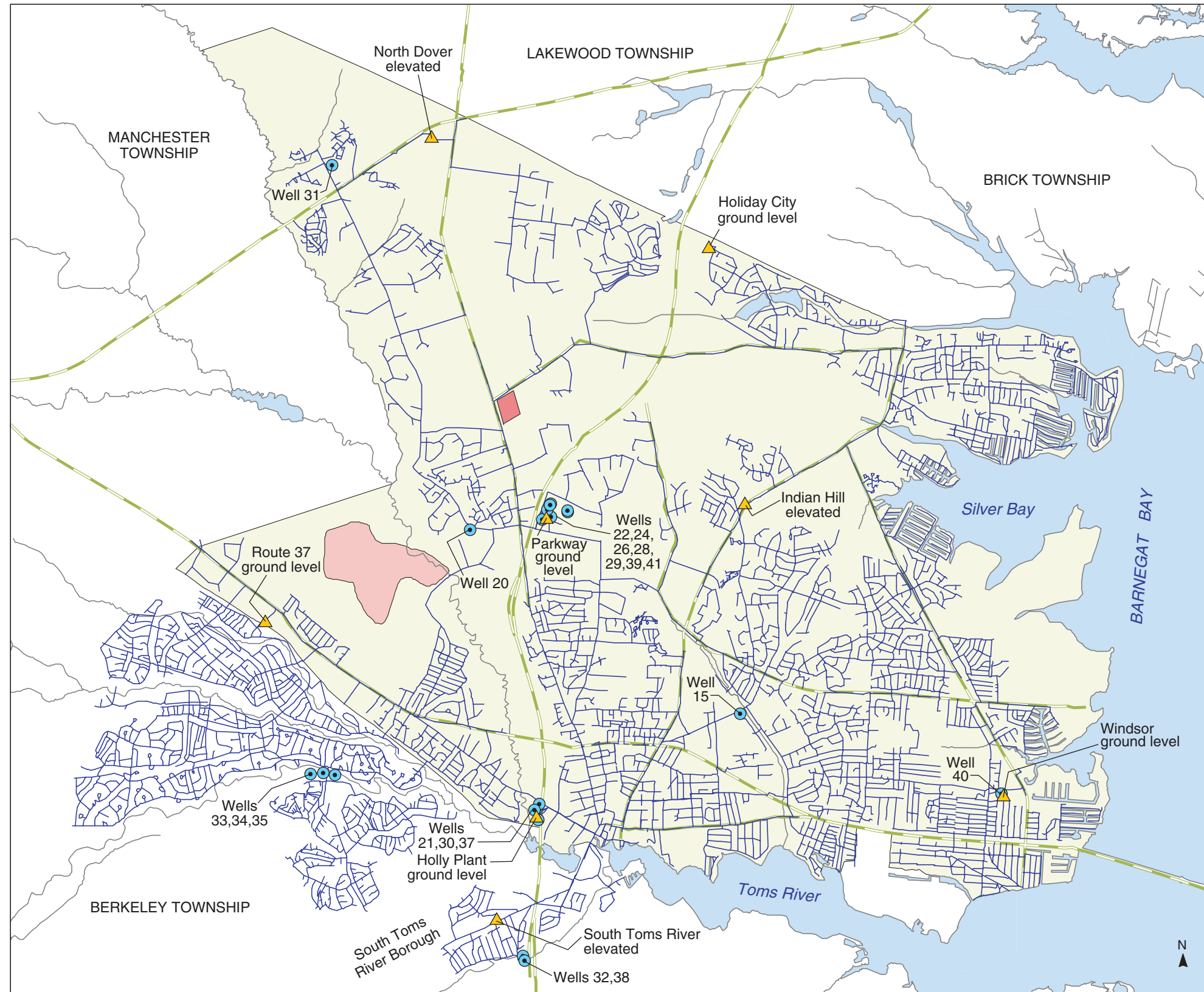
PLATE 34. WATER-DISTRIBUTION SYSTEM SERVING THE DOVER TOWNSHIP AREA, NEW JERSEY, 1993 By Morris L. Maslia, Jason B. Sautner, Mustafa M. Aral, Richard E. Gillig, Juan J. Reyes, and Robert C. Williams
