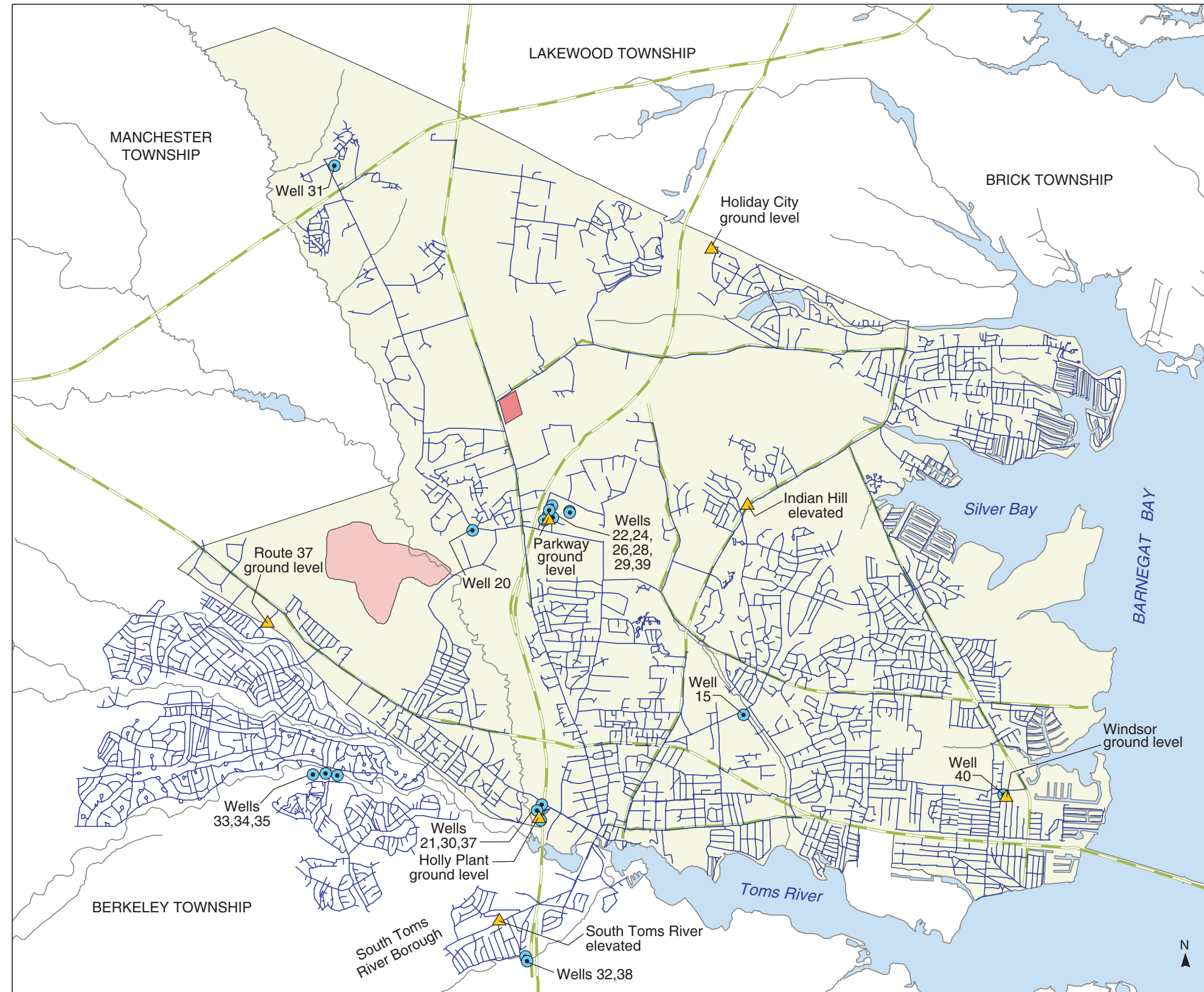
PLATE 32. WATER-DISTRIBUTION SYSTEM SERVING THE DOVER TOWNSHIP AREA, NEW JERSEY, 1991 By Morris L. Maslia, Jason B. Sautner, Mustafa M. Aral, Richard E. Gillig, Juan J. Reyes, and Robert C. Williams
