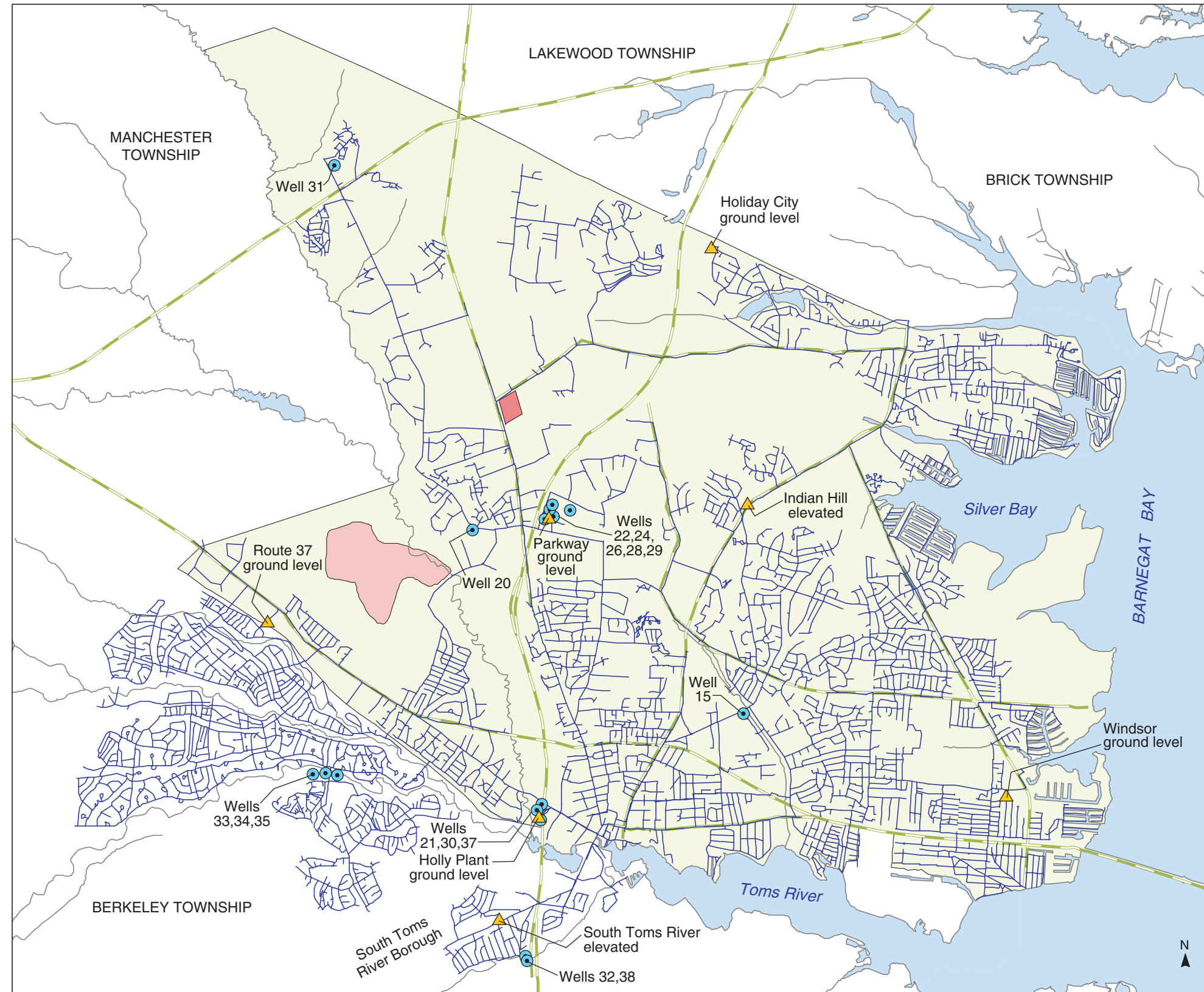
PLATE 31. WATER-DISTRIBUTION SYSTEM SERVING THE DOVER TOWNSHIP AREA, NEW JERSEY, 1990 By Morris L. Maslia, Jason B. Sautner, Mustafa M. Aral, Richard E. Gillig, Juan J. Reyes, and Robert C. Williams
