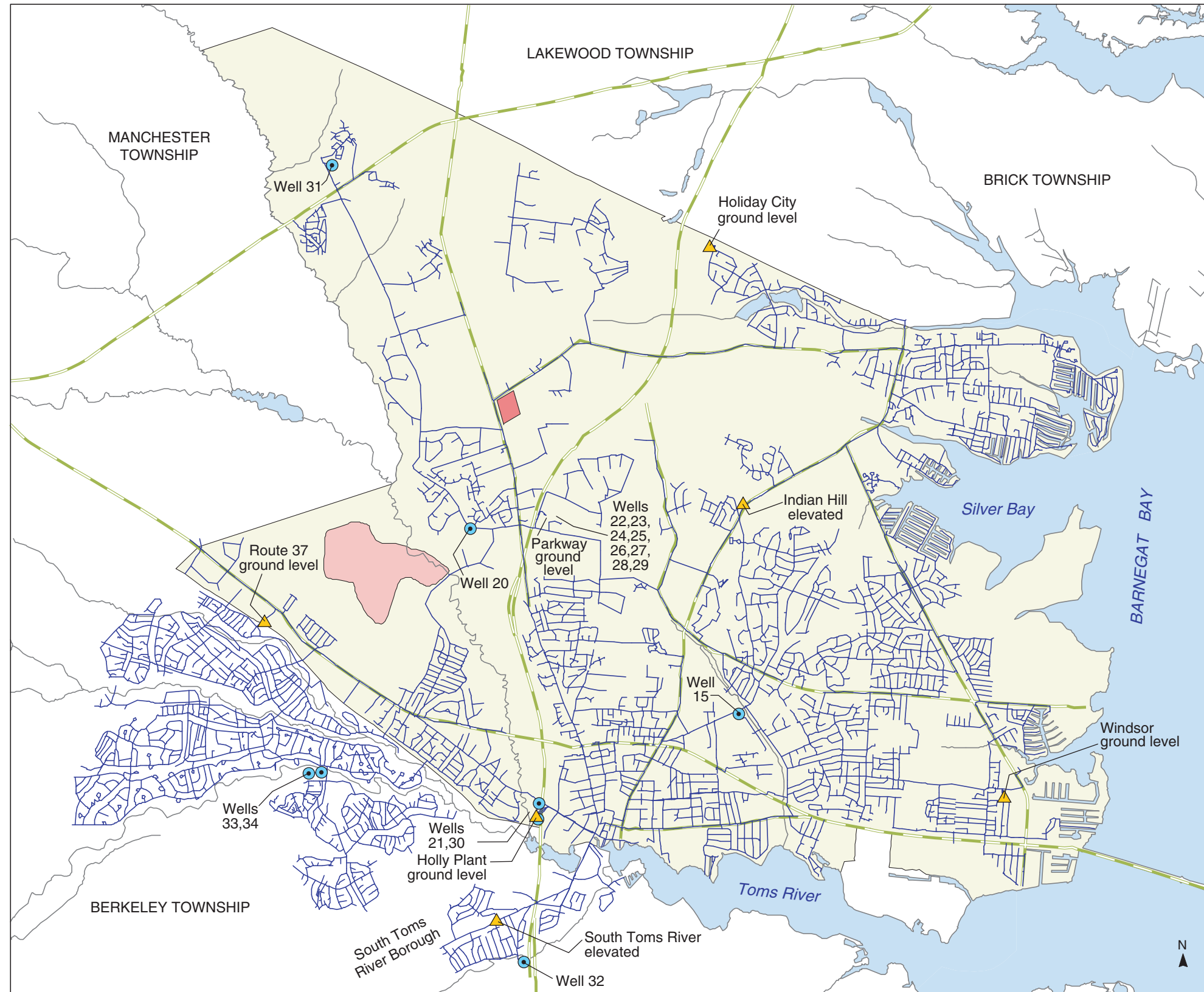
PLATE 28. WATER-DISTRIBUTION SYSTEM SERVING THE DOVER TOWNSHIP AREA, NEW JERSEY, 1987 By Morris L. Maslia, Jason B. Sautner, Mustafa M. Aral, Richard E. Gillig, Juan J. Reyes, and Robert C. Williams
