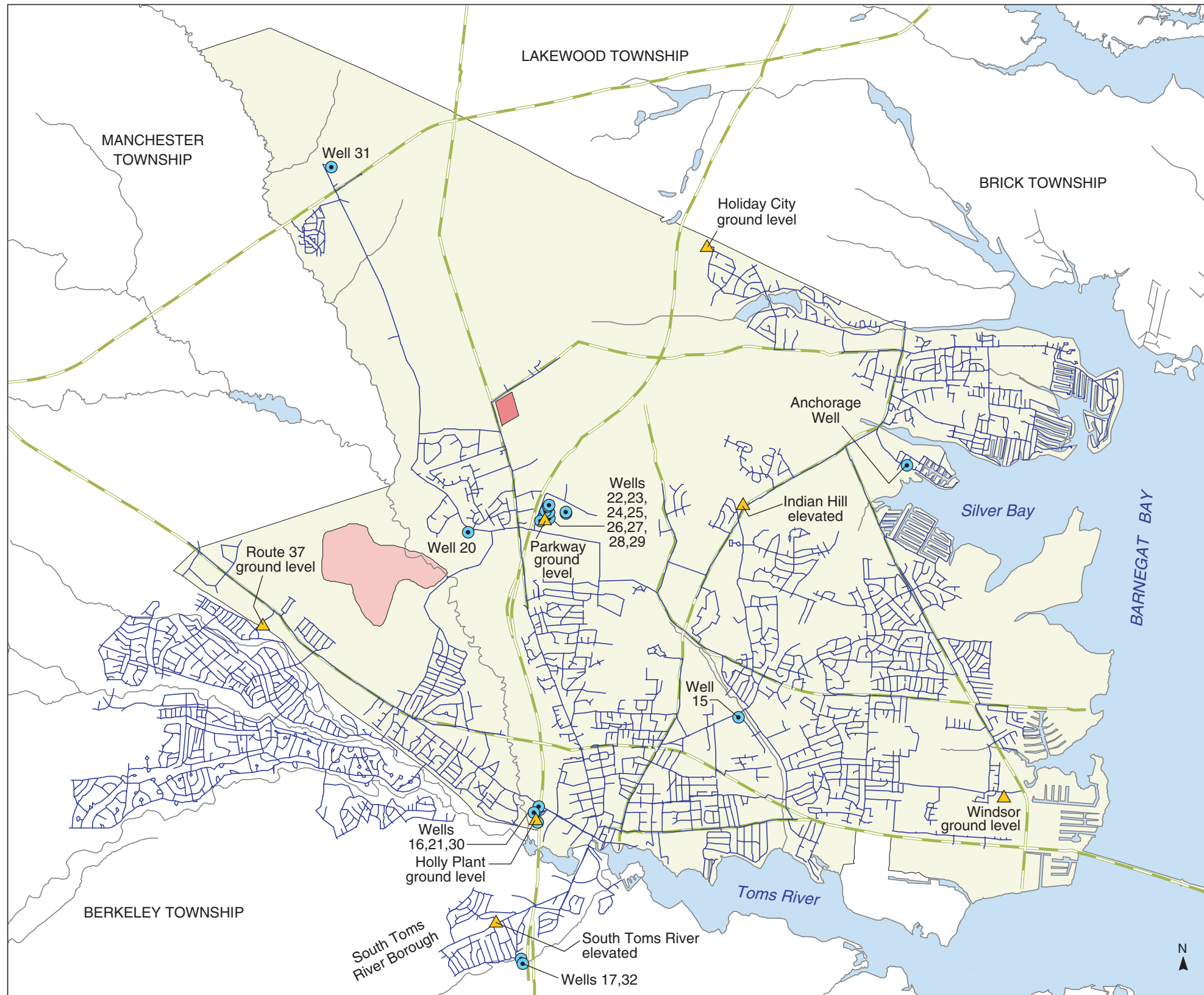
PLATE 25. WATER-DISTRIBUTION SYSTEM SERVING THE DOVER TOWNSHIP AREA, NEW JERSEY, 1984 By Morris L. Maslia, Jason B. Sautner, Mustafa M. Aral, Richard E. Gillig, Juan J. Reyes, and Robert C. Williams
