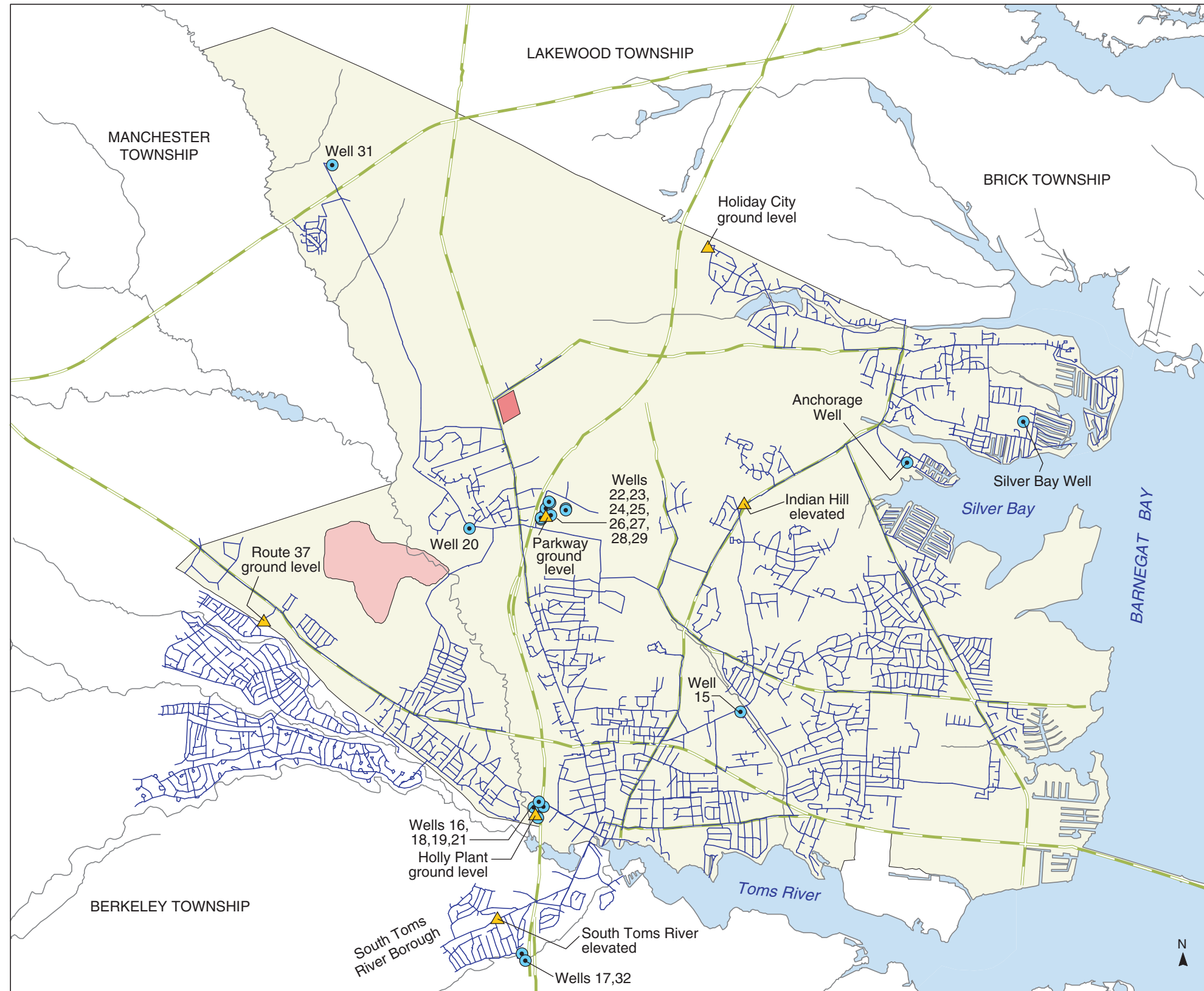
PLATE 21. WATER-DISTRIBUTION SYSTEM SERVING THE DOVER TOWNSHIP AREA, NEW JERSEY, 1980 By Morris L. Maslia, Jason B. Sautner, Mustafa M. Aral, Richard E. Gillig, Juan J. Reyes, and Robert C. Williams
