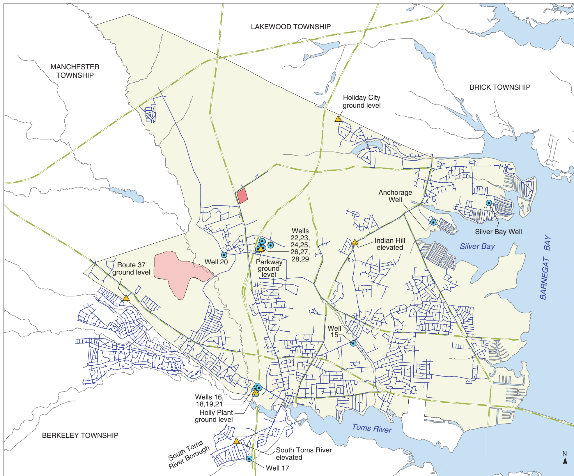
PLATE 19. WATER-DISTRIBUTION SYSTEM SERVING THE DOVER TOWNSHIP AREA, NEW JERSEY, 1978 By Morris L. Maslia, Jason B. Sautner, Mustafa M. Aral, Richard E. Gillig, Juan J. Reyes, and Robert C. Williams
