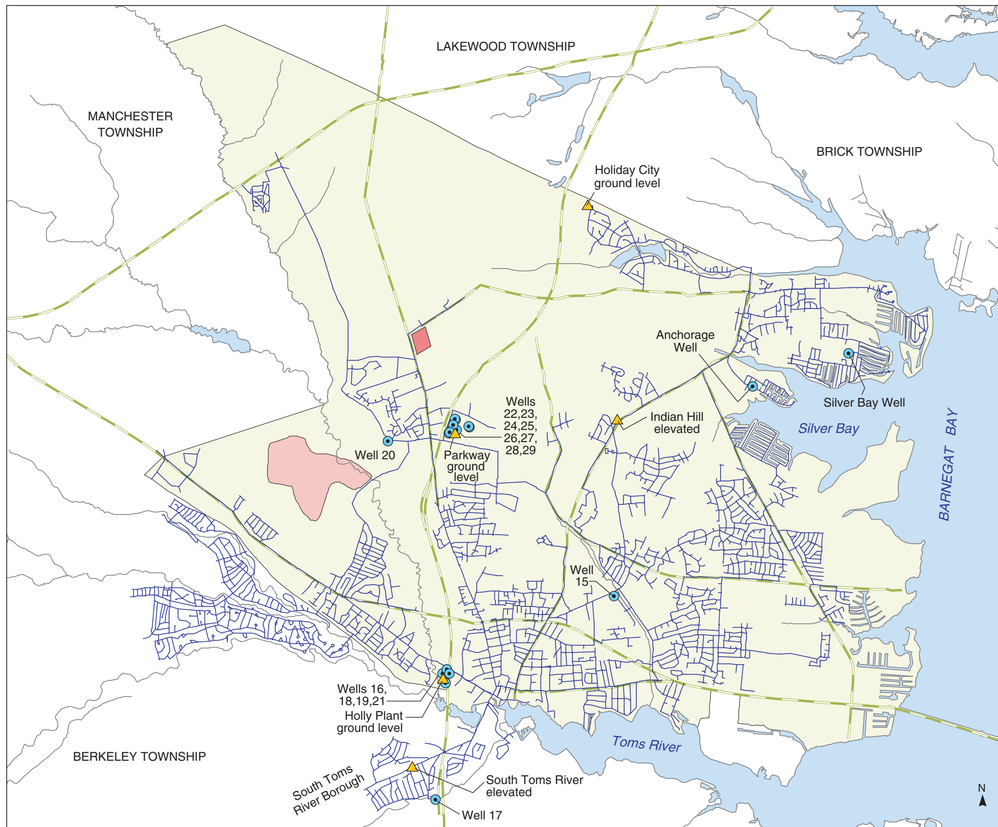
PLATE 18. WATER-DISTRIBUTION SYSTEM SERVING THE DOVER TOWNSHIP AREA, NEW JERSEY, 1977 By Morris L. Maslia, Jason B. Sautner, Mustafa M. Aral, Richard E. Gillig, Juan J. Reyes, and Robert C. Williams
