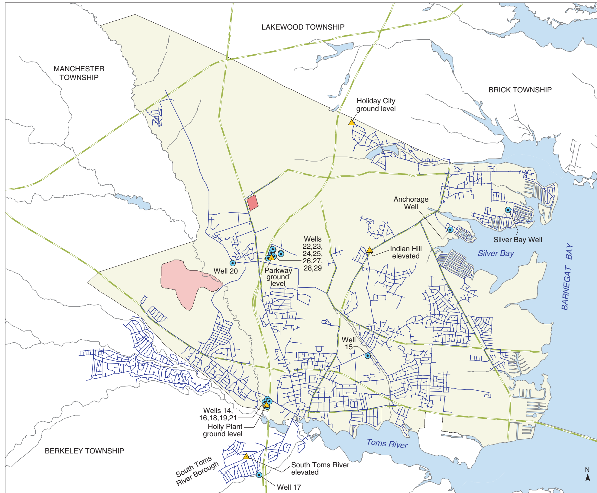
PLATE 16. WATER-DISTRIBUTION SYSTEM SERVING THE DOVER TOWNSHIP AREA, NEW JERSEY, 1975 By Morris L. Maslia, Jason B. Sautner, Mustafa M. Aral, Richard E. Gillig, Juan J. Reyes, and Robert C. Williams
